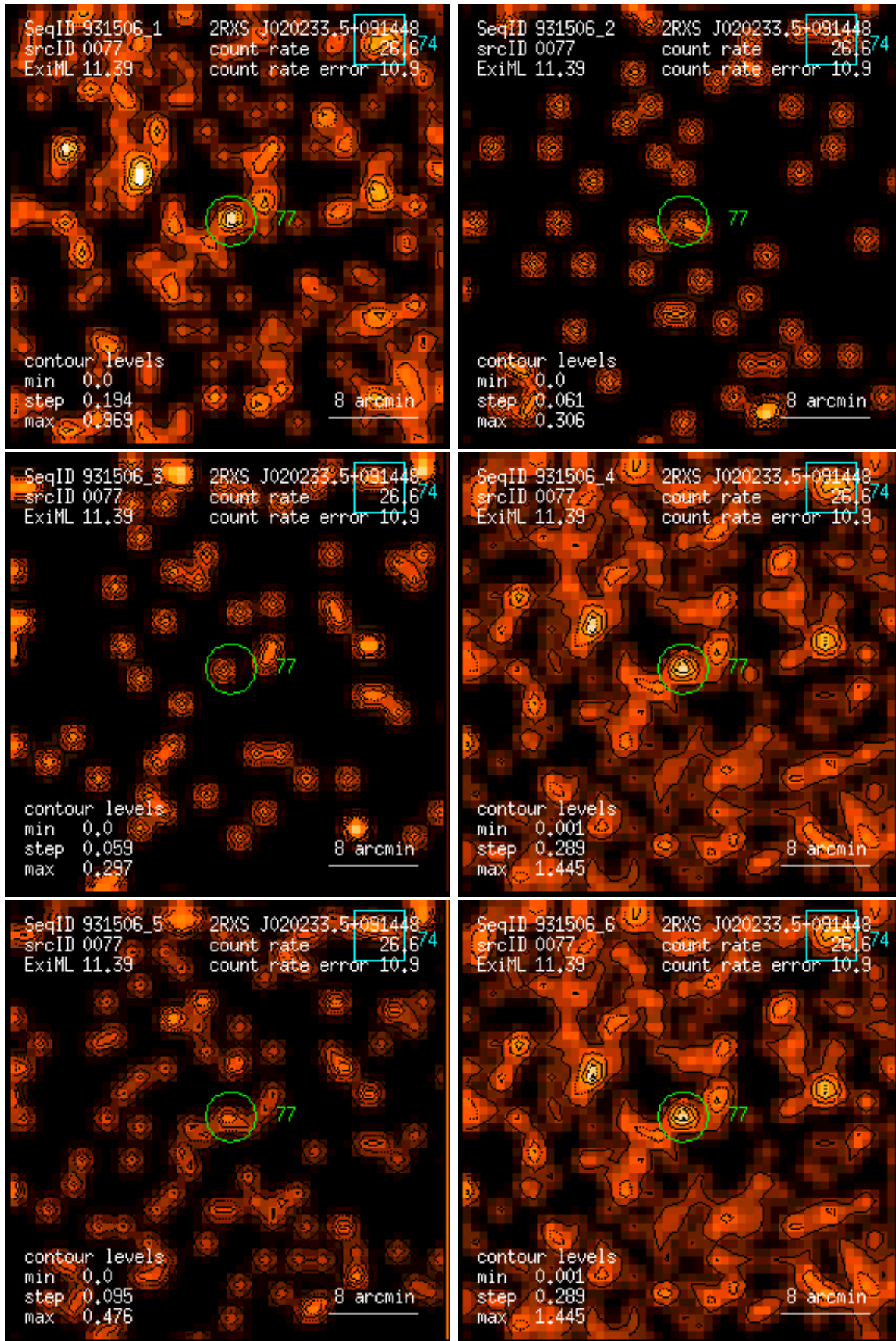
Figure 77: RASS 931506: detection 0077: band rate images, Gaussian filter: (1) PSPC channels 11 – 41, (2) 52 – 90, (3) 91 – 201, (4) 11 – 235, (5) 52 – 201, (6) 11 – 201. Broad band rates in counts/ks. Band rate contour levels in counts/ks/arcmin 2 .
