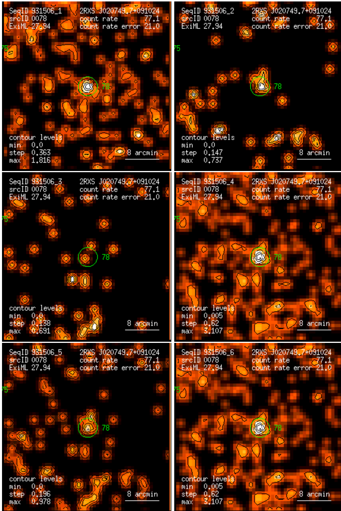
Figure 78: RASS 931506: detection 0078: band rate images, Gaussian filter: (1) PSPC channels 11 – 41, (2) 52 – 90, (3) 91 – 201, (4) 11 – 235, (5) 52 – 201, (6) 11 – 201. Broad band rates in counts/ks. Band rate contour levels in counts/ks/arcmin 2 .
