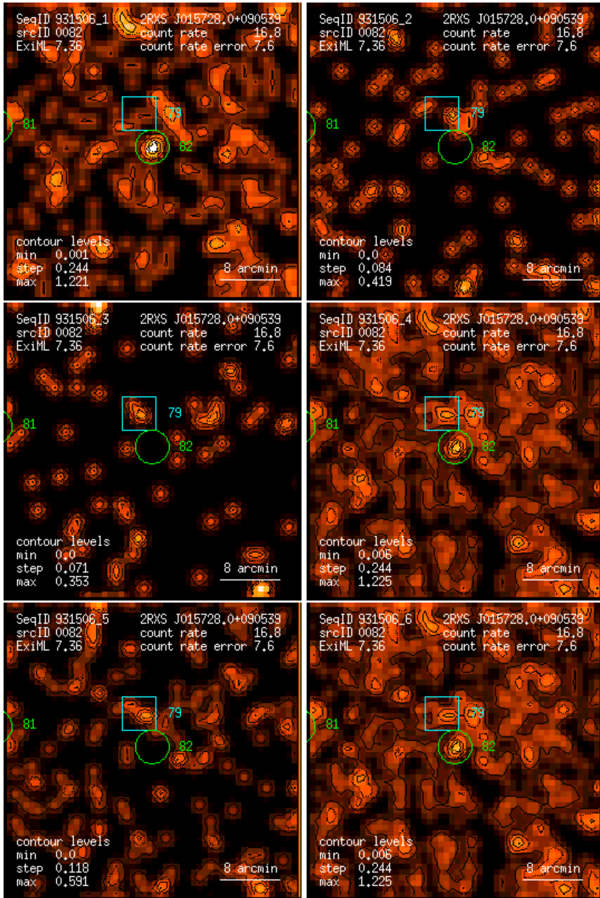
Figure 82: RASS 931506: detection 0082: band rate images, Gaussian filter: (1) PSPC channels 11 – 41, (2) 52 – 90, (3) 91 – 201, (4) 11 – 235, (5) 52 – 201, (6) 11 – 201. Broad band rates in counts/ks. Band rate contour levels in counts/ks/arcmin 2 .
