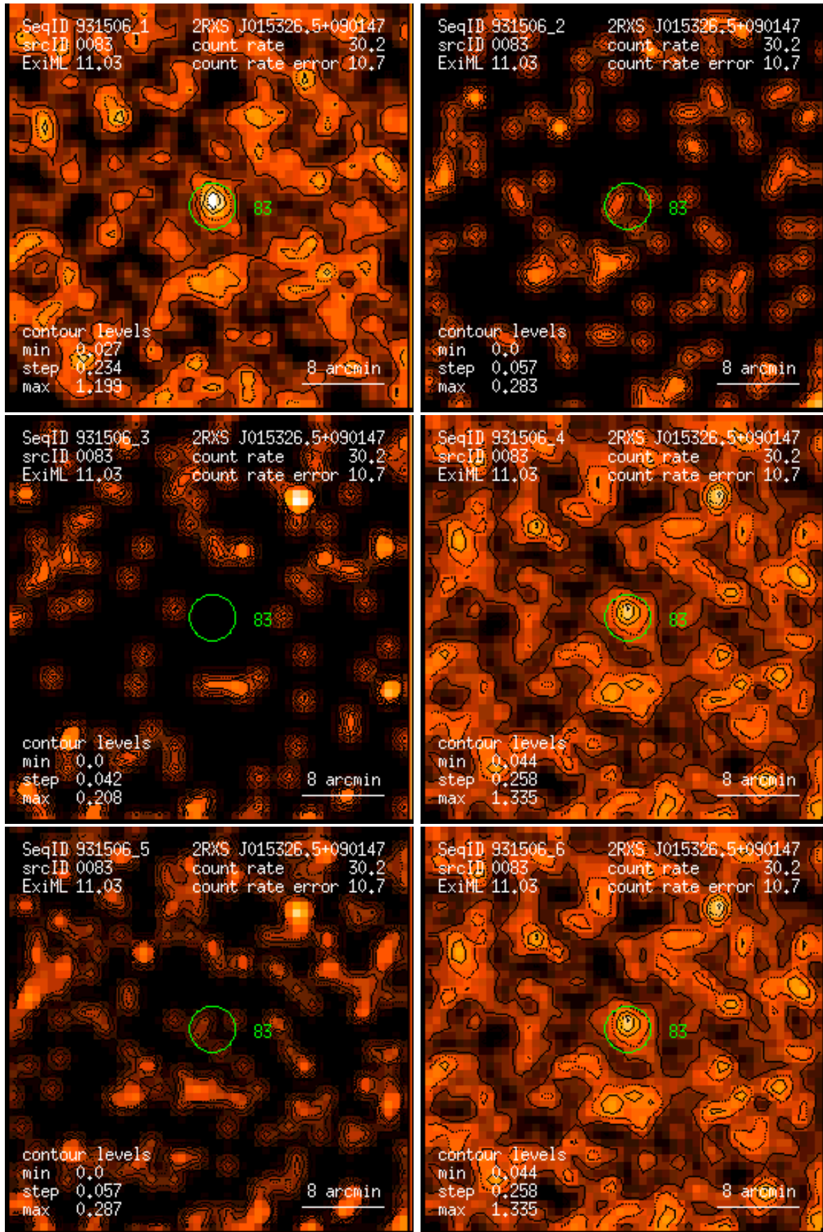
Figure 83: RASS 931506: detection 0083: band rate images, Gaussian filter: (1) PSPC channels 11 – 41, (2) 52 – 90, (3) 91 – 201, (4) 11 – 235, (5) 52 – 201, (6) 11 – 201. Broad band rates in counts/ks. Band rate contour levels in counts/ks/arcmin 2 .
