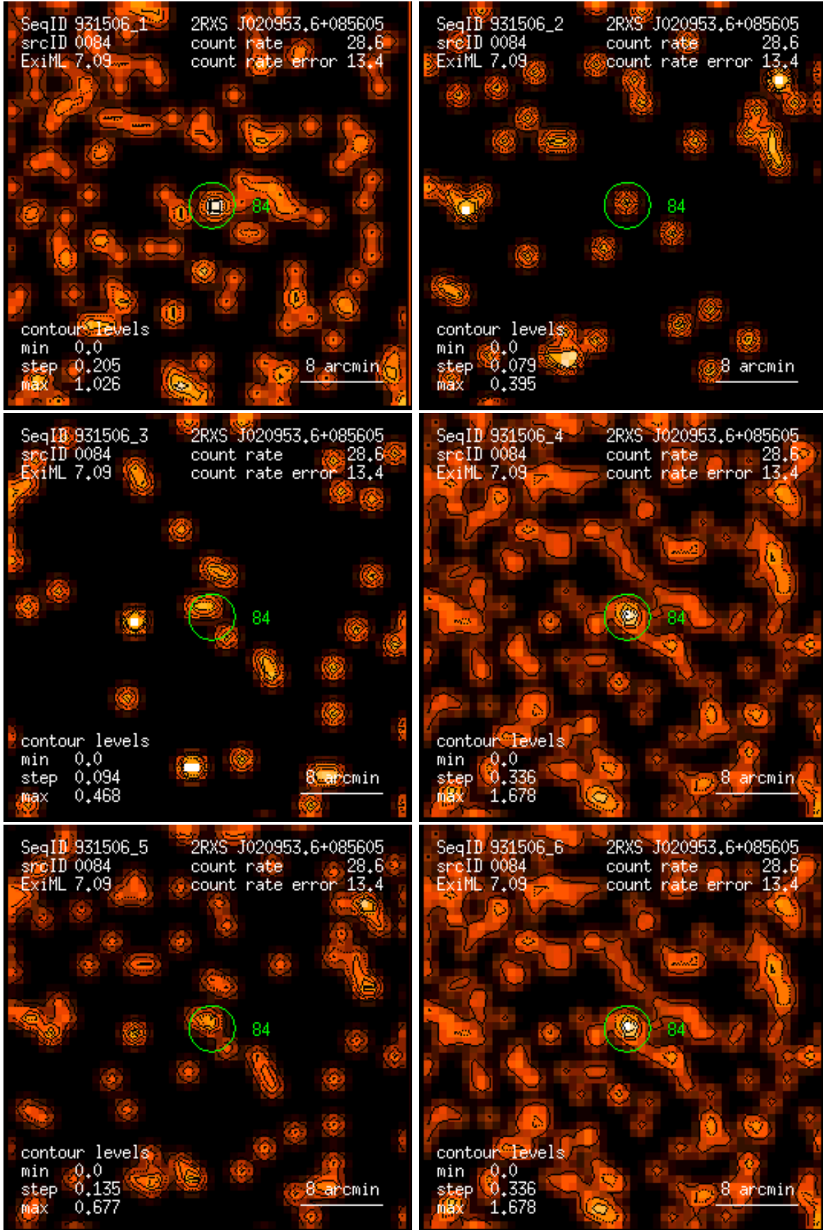
Figure 84: RASS 931506: detection 0084: band rate images, Gaussian filter: (1) PSC channels 11 – 41, (2) 52 – 90, (3) 91 – 201, (4) 11 – 235, (5) 52 – 201, (6) 11 – 201. Broad band rates in counts/ks. Band rate contour levels in counts/ks/arcmin 2 .
