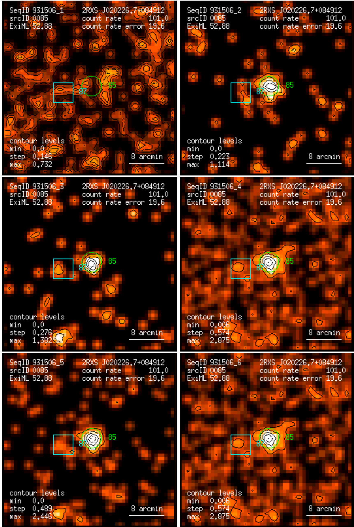
Figure 85: RASS 931506: detection 0085: band rate images, Gaussian filter: (1) PSPC channels 11 – 41, (2) 52 – 90, (3) 91 – 201, (4) 11 – 235, (5) 52 – 201, (6) 11 – 201. Broad band rates in counts/ks. Band rate contour levels in counts/ks/arcmin 2 .
