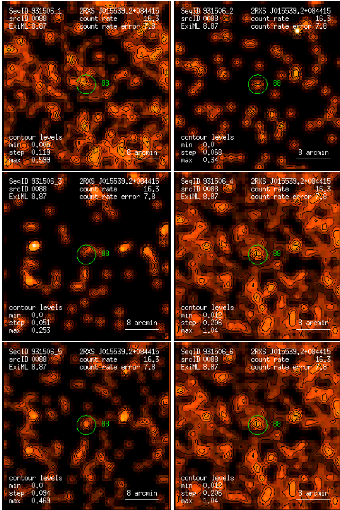
Figure 88: RASS 931506: detection 0088: band rate images, Gaussian filter: (1) PSPC channels 11 – 41, (2) 52 – 90, (3) 91 – 201, (4) 11 – 235, (5) 52 – 201, (6) 11 – 201. Broad band rates in counts/ks. Band rate contour levels in counts/ks/arcmin 2 .
