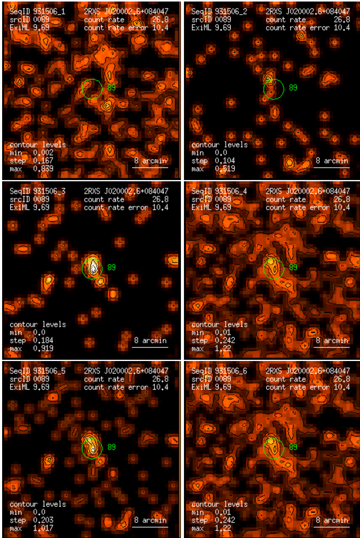
Figure 89: RASS 931506: detection 0089: band rate images, Gaussian filter: (1) PSPC channels 11 – 41, (2) 52 – 90, (3) 91 – 201, (4) 11 – 235, (5) 52 – 201, (6) 11 – 201. Broad band rates in counts/ks. Band rate contour levels in counts/ks/arcmin 2 .
