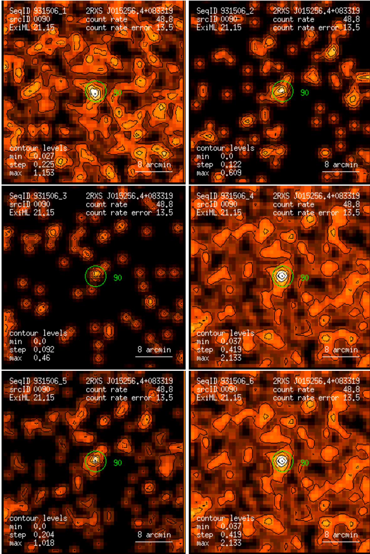
Figure 90: RASS 931506: detection 0090: band rate images, Gaussian filter: (1) PSPC channels 11 – 41, (2) 52 – 90, (3) 91 – 201, (4) 11 – 235, (5) 52 – 201, (6) 11 – 201. Broad band rates in counts/ks. Band rate contour levels in counts/ks/arcmin 2 .
