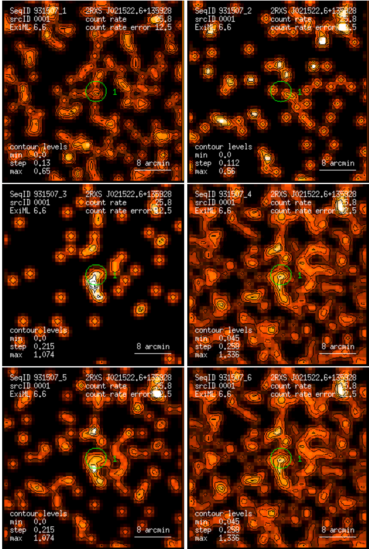
Figure 1: RASS 931507: detection 0001: band rate images, Gaussian filter: (1) PSPC channels 11 – 41, (2) 52 – 90, (3) 91 – 201, (4) 11 – 235, (5) 52 – 201, (6) 11 – 201. Broad band rates in counts/ks. Band rate contour levels in counts/ks/arcmin 2 .
