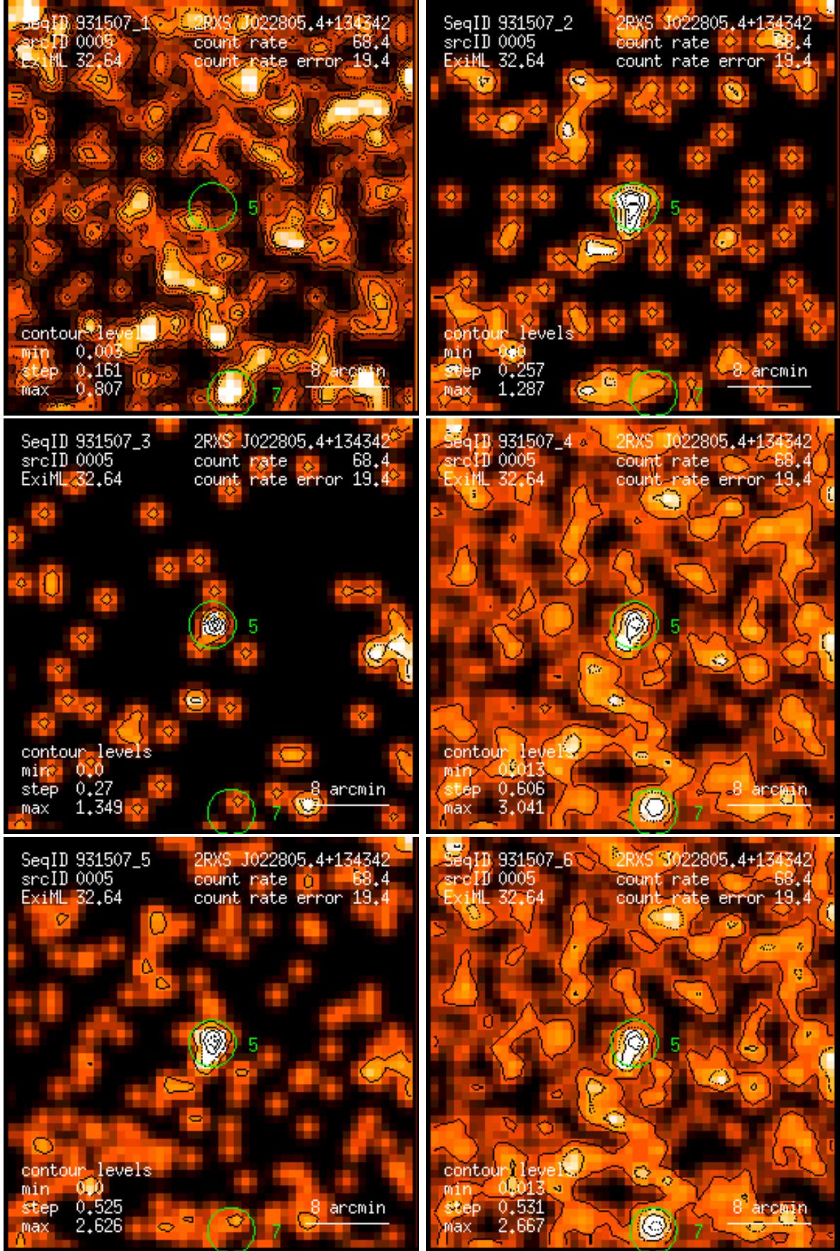
Figure 5: RASS 931507: detection 0005: band rate images, Gaussian filter: (1) PSPC channels 11 – 41, (2) 52 – 90, (3) 91 – 201, (4) 11 – 235, (5) 52 – 201, (6) 11 – 201. Broad band rates in counts/ks. Band rate contour levels in counts/ks/arcmin 2 .
