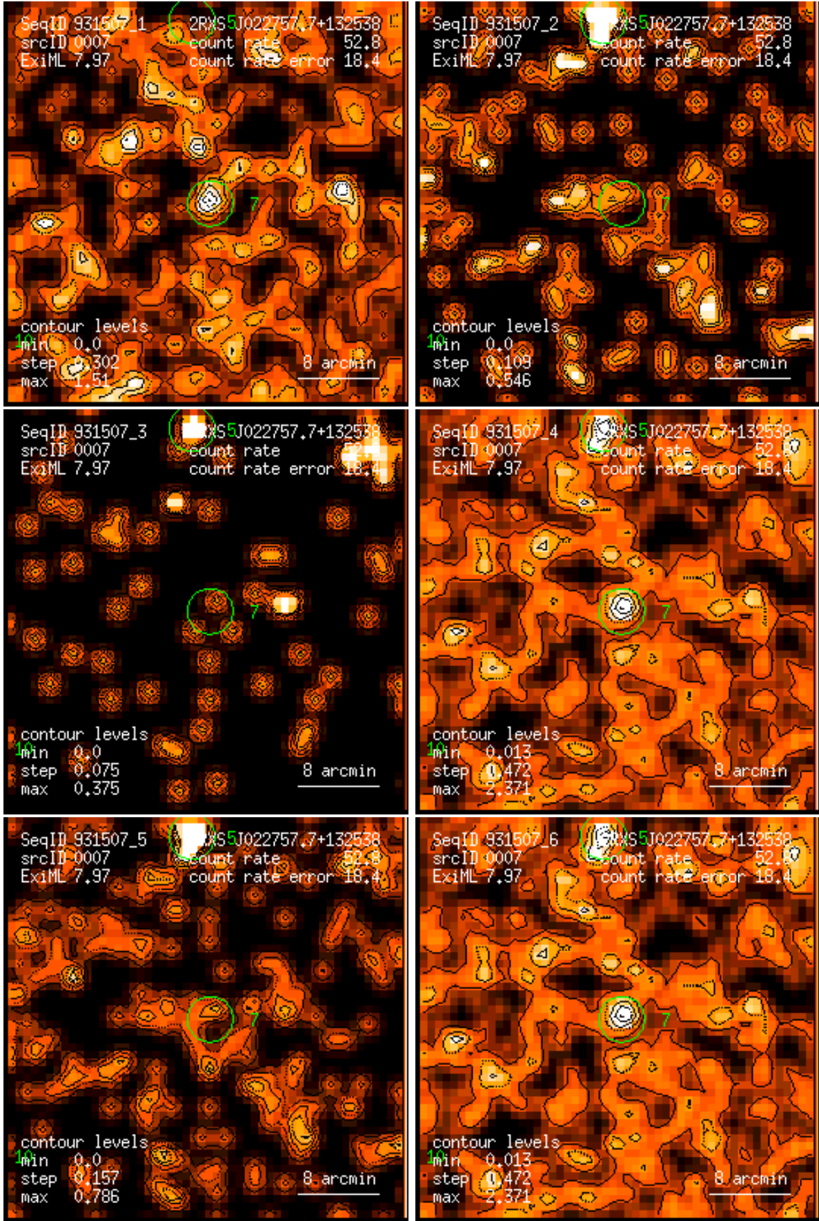
Figure 7: RASS 931507: detection 0007: band rate images, Gaussian filter: (1) PSPC channels 11 – 41, (2) 52 – 90, (3) 91 – 201, (4) 11 – 235, (5) 52 – 201, (6) 11 – 201. Broad band rates in counts/ks. Band rate contour levels in counts/ks/arcmin 2 .
