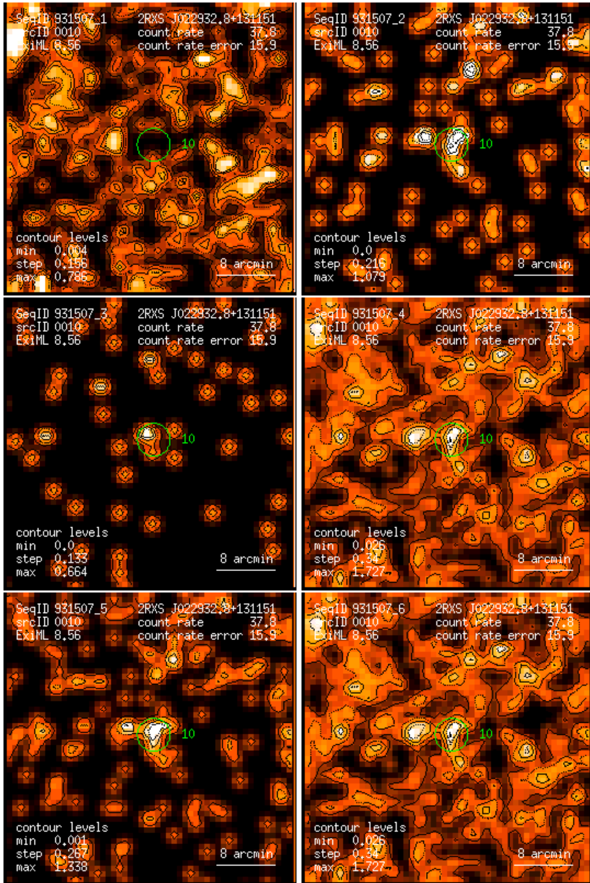
Figure 10: RASS 931507: detection 0010: band rate images, Gaussian filter: (1) PSPC channels 11 – 41, (2) 52 – 90, (3) 91 – 201, (4) 11 – 235, (5) 52 – 201, (6) 11 – 201. Broad band rates in counts/ks. Band rate contour levels in counts/ks/arcmin 2 .
