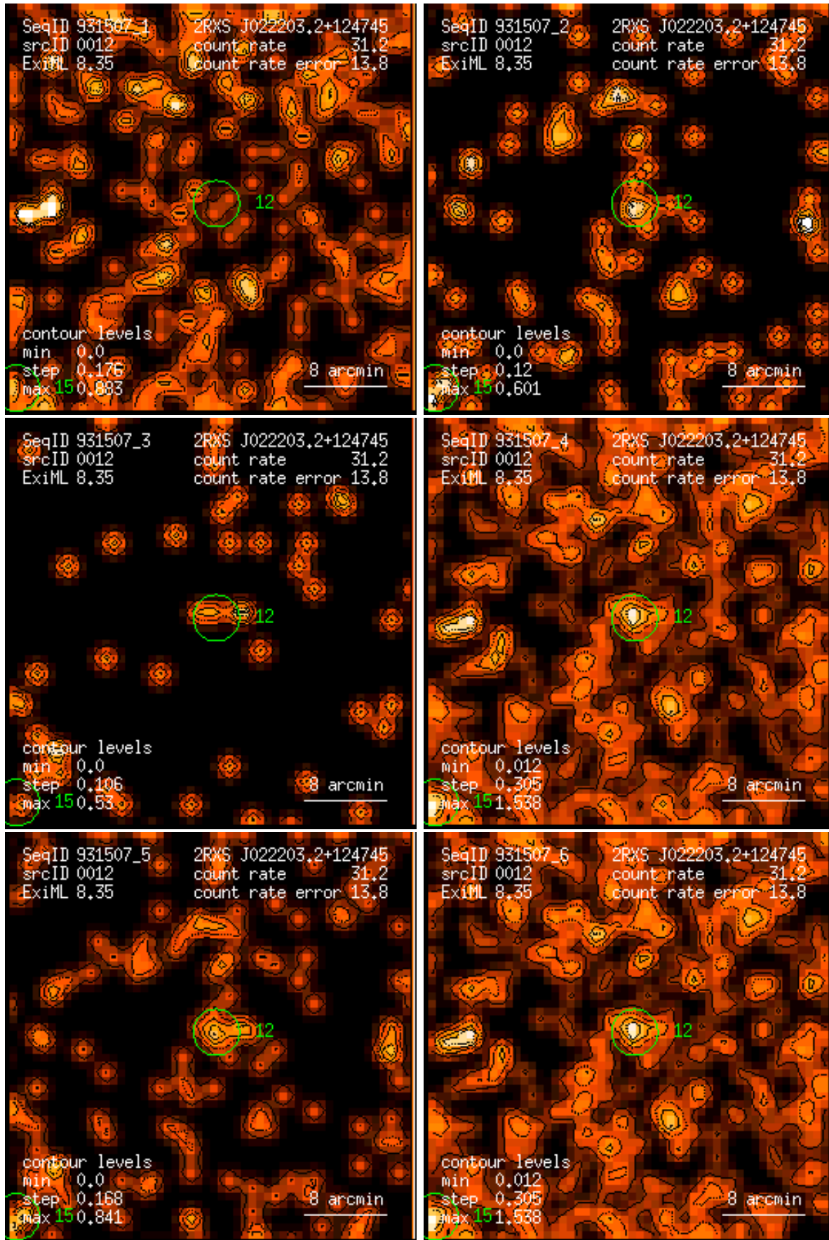
Figure 12: RASS 931507: detection 0012: band rate images, Gaussian filter: (1) PSPC channels 11 – 41, (2) 52 – 90, (3) 91 – 201, (4) 11 – 235, (5) 52 – 201, (6) 11 – 201. Broad band rates in counts/ks. Band rate contour levels in counts/ks/arcmin 2 .
