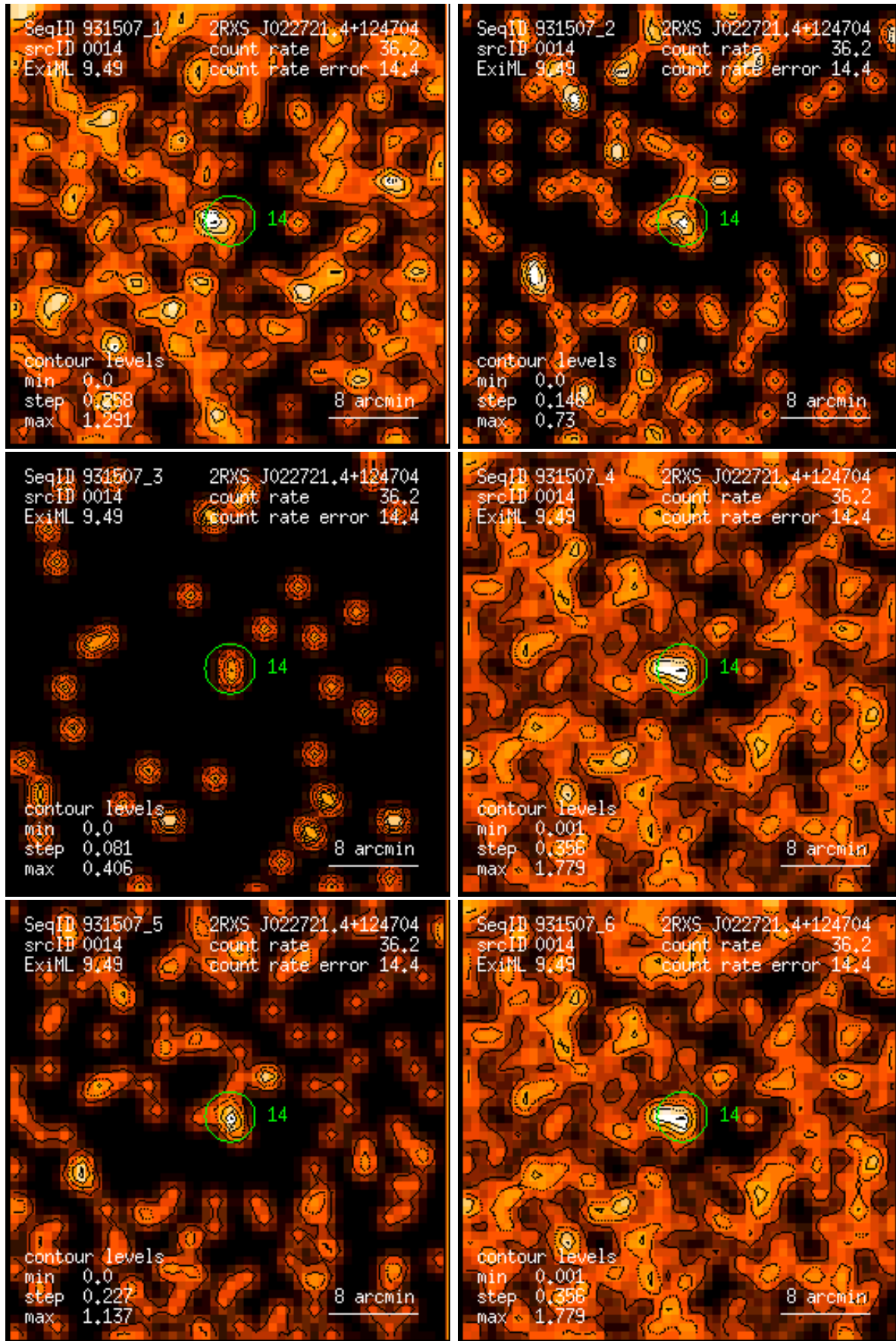
Figure 14: RASS 931507: detection 0014: band rate images, Gaussian filter: (1) PSPC channels 11 – 41, (2) 52 – 90, (3) 91 – 201, (4) 11 – 235, (5) 52 – 201, (6) 11 – 201. Broad band rates in counts/ks. Band rate contour levels in counts/ks/arcmin 2 .
