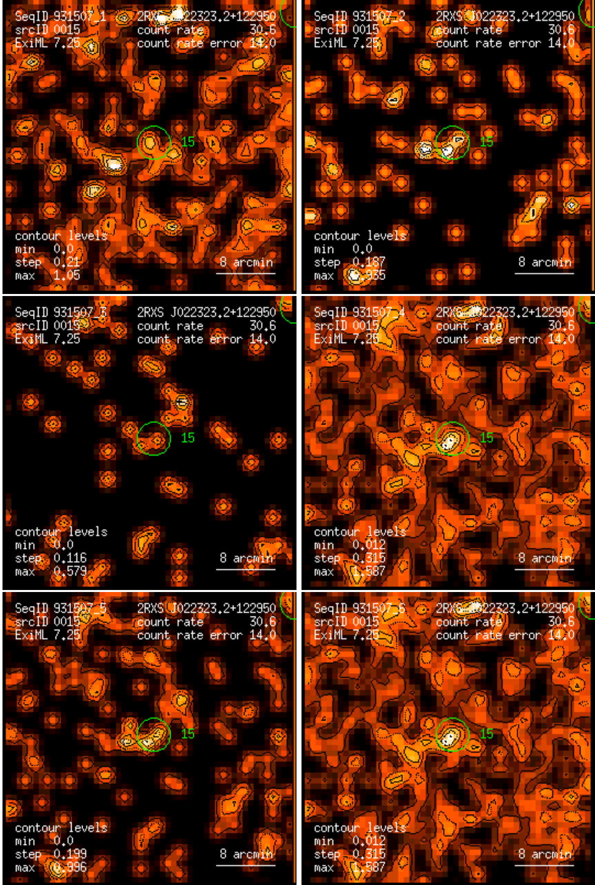
Figure 15: RASS 931507: detection 0015: band rate images, Gaussian filter: (1) PSPC channels 11 – 41, (2) 52 – 90, (3) 91 – 201, (4) 11 – 235, (5) 52 – 201, (6) 11 – 201. Broad band rates in counts/ks. Band rate contour levels in counts/ks/arcmin 2 .
