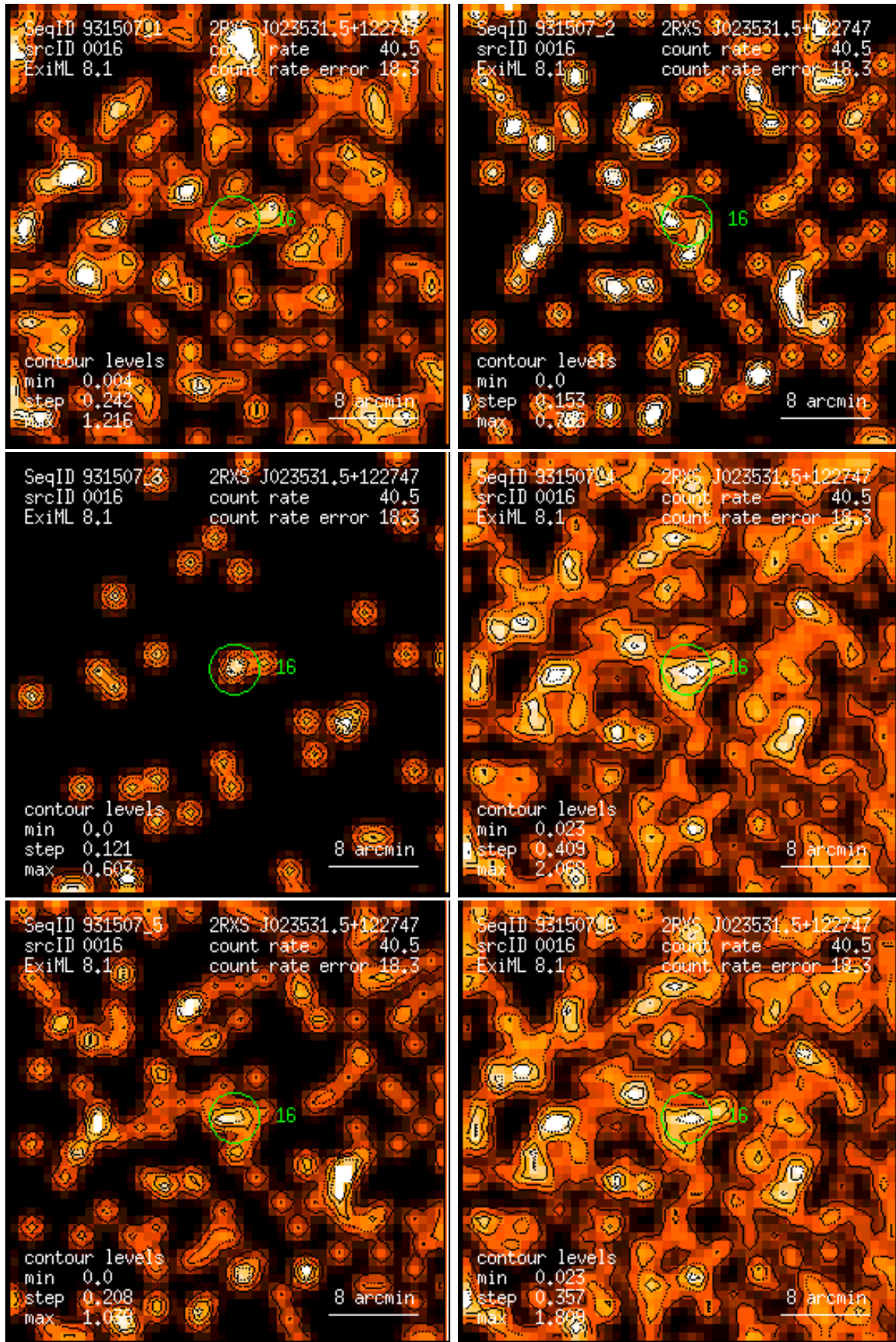
Figure 16: RASS 931507: detection 0016: band rate images, Gaussian filter: (1) PSPC channels 11 – 41, (2) 52 – 90, (3) 91 – 201, (4) 11 – 235, (5) 52 – 201, (6) 11 – 201. Broad band rates in counts/ks. Band rate contour levels in counts/ks/arcmin 2 .
