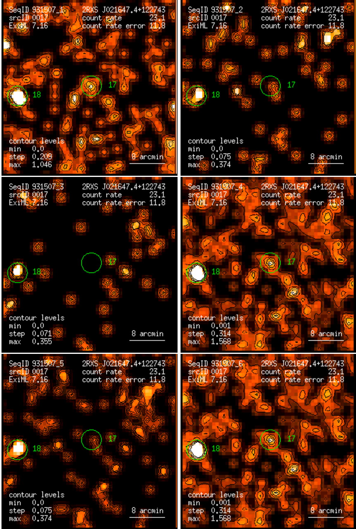
Figure 17: RASS 931507: detection 0017: band rate images, Gaussian filter: (1) PSPC channels 11 – 41, (2) 52 – 90, (3) 91 – 201, (4) 11 – 235, (5) 52 – 201, (6) 11 – 201. Broad band rates in counts/ks. Band rate contour levels in counts/ks/arcmin 2 .
