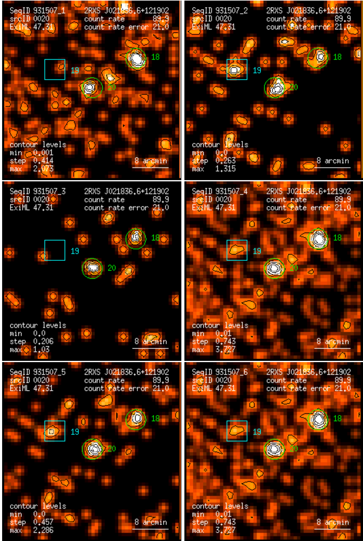
Figure 20: RASS 931507: detection 0020: band rate images, Gaussian filter: (1) PSPC channels 11 – 41, (2) 52 – 90, (3) 91 – 201, (4) 11 – 235, (5) 52 – 201, (6) 11 – 201. Broad band rates in counts/ks. Band rate contour levels in counts/ks/arcmin 2 .
