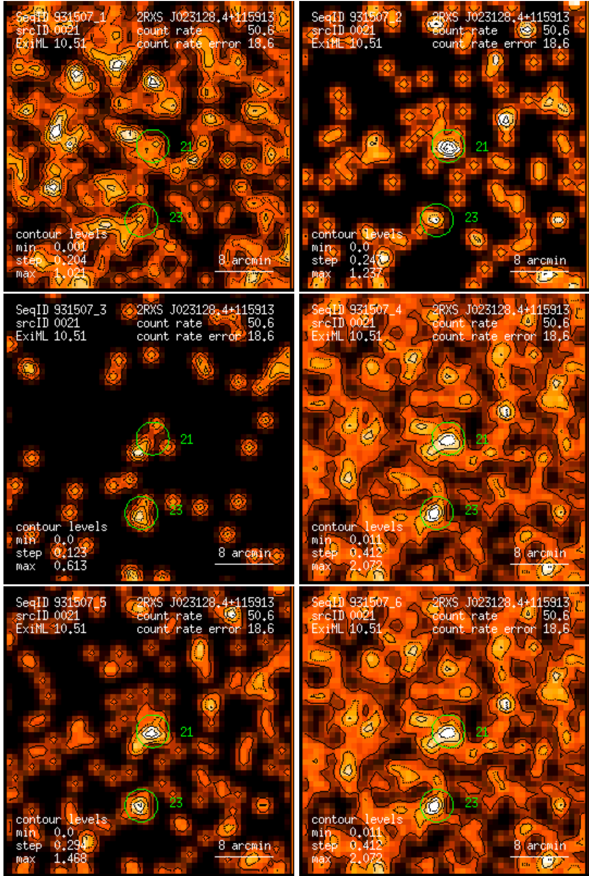
Figure 21: RASS 931507: detection 0021: band rate images, Gaussian filter: (1) PSPC channels 11 – 41, (2) 52 – 90, (3) 91 – 201, (4) 11 – 235, (5) 52 – 201, (6) 11 – 201. Broad band rates in counts/ks. Band rate contour levels in counts/ks/arcmin 2 .
