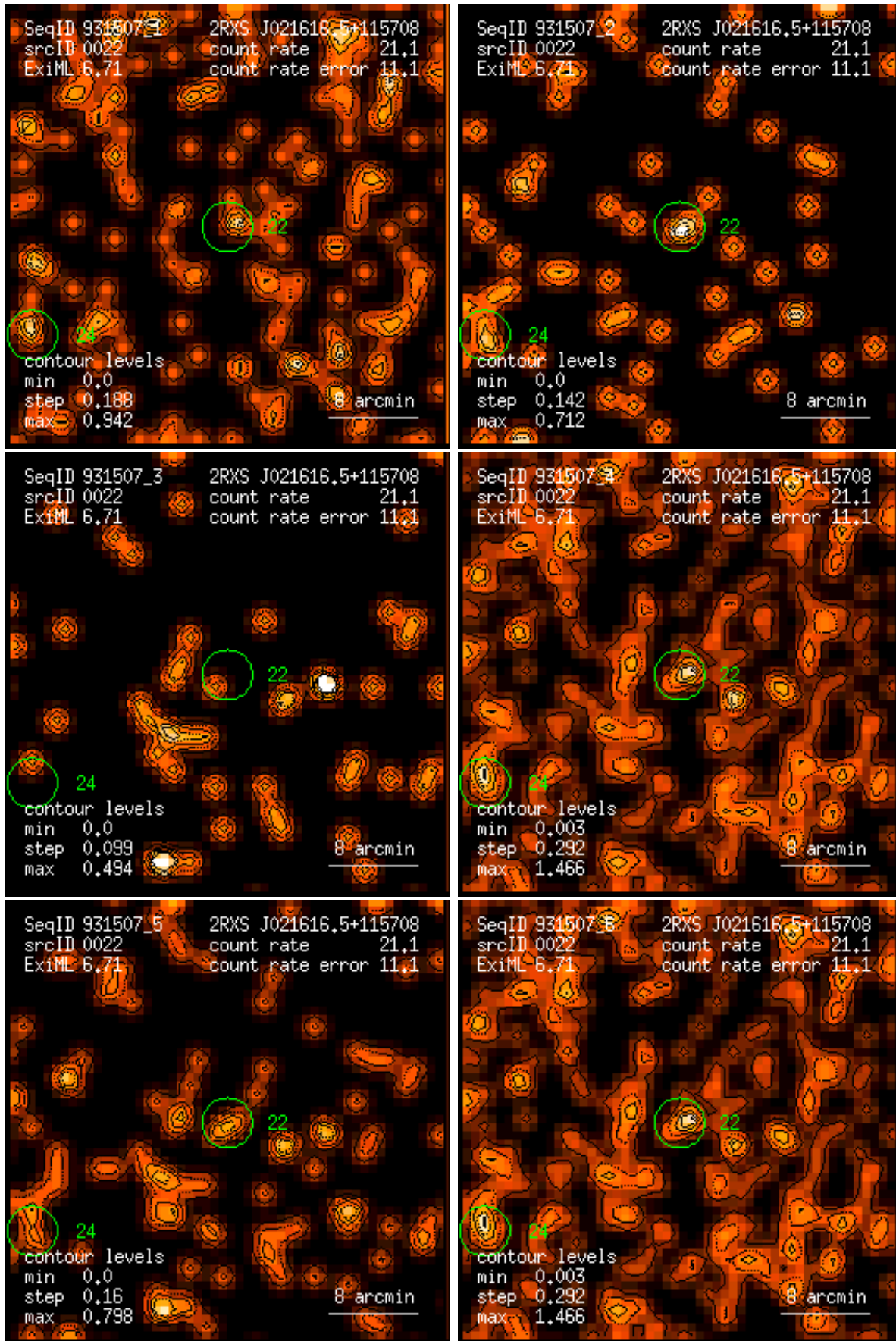
Figure 22: RASS 931507: detection 0022: band rate images, Gaussian filter: (1) PSPC channels 11 – 41, (2) 52 – 90, (3) 91 – 201, (4) 11 – 235, (5) 52 – 201, (6) 11 – 201. Broad band rates in counts/ks. Band rate contour levels in counts/ks/arcmin 2 .
