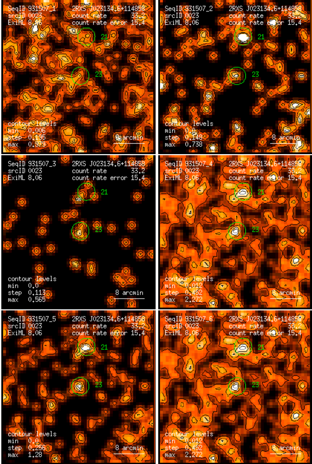
Figure 23: RASS 931507: detection 0023: band rate images, Gaussian filter: (1) PSPC channels 11 – 41, (2) 52 – 90, (3) 91 – 201, (4) 11 – 235, (5) 52 – 201, (6) 11 – 201. Broad band rates in counts/ks. Band rate contour levels in counts/ks/arcmin 2 .
