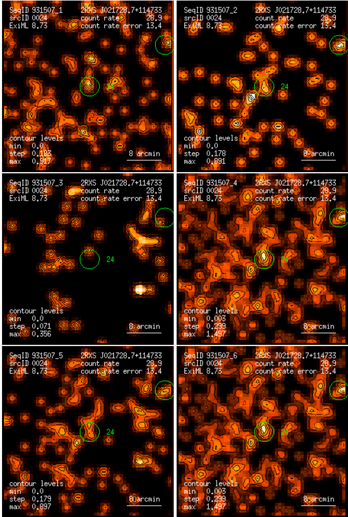
Figure 24: RASS 931507: detection 0024: band rate images, Gaussian filter: (1) PSPC channels 11 – 41, (2) 52 – 90, (3) 91 – 201, (4) 11 – 235, (5) 52 – 201, (6) 11 – 201. Broad band rates in counts/ks. Band rate contour levels in counts/ks/arcmin 2 .
