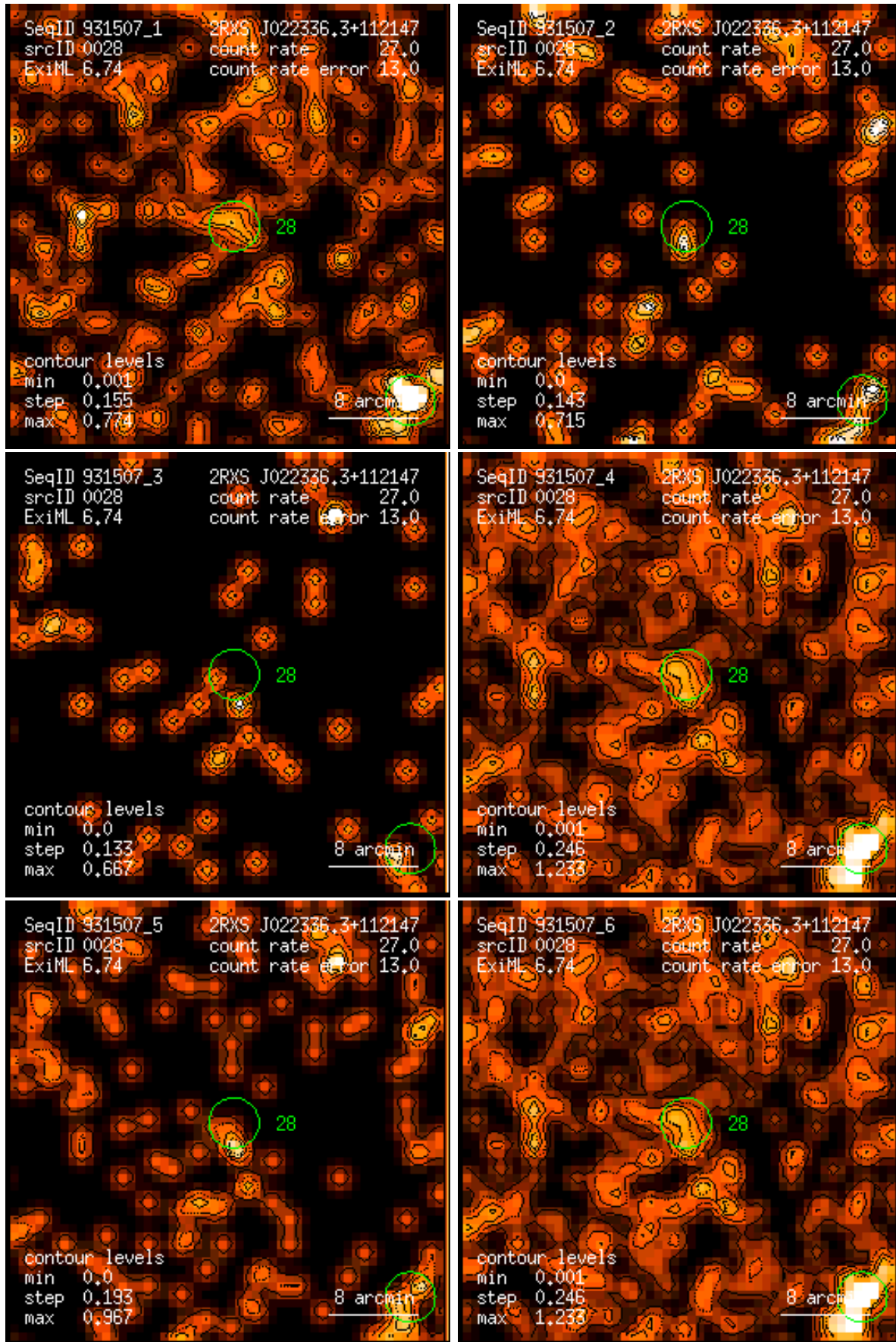
Figure 28: RASS 931507: detection 0028: band rate images, Gaussian filter: (1) PSPC channels 11 – 41, (2) 52 – 90, (3) 91 – 201, (4) 11 – 235, (5) 52 – 201, (6) 11 – 201. Broad band rates in counts/ks. Band rate contour levels in counts/ks/arcmin 2 .
