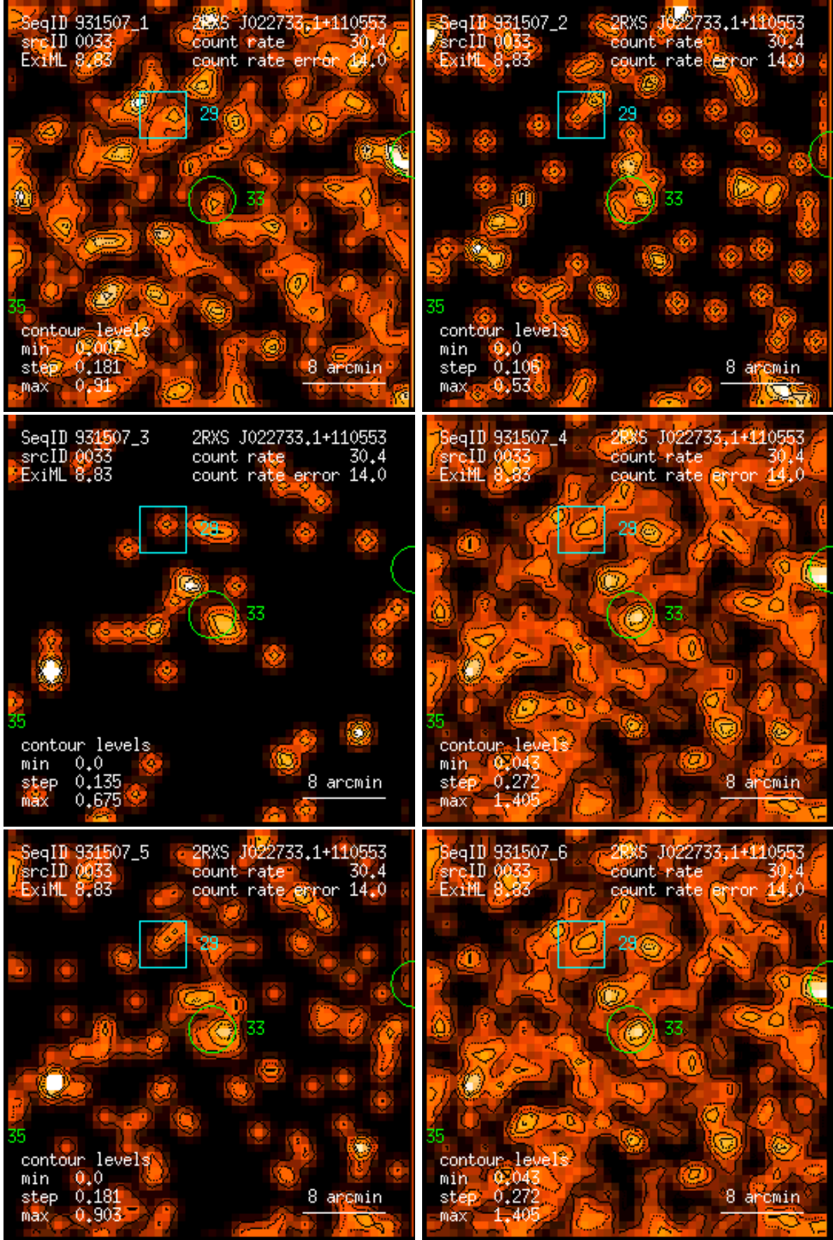
Figure 33: RASS 931507: detection 0033: band rate images, Gaussian filter: (1) PSPC channels 11 – 41, (2) 52 – 90, (3) 91 – 201, (4) 11 – 235, (5) 52 – 201, (6) 11 – 201. Broad band rates in counts/ks. Band rate contour levels in counts/ks/arcmin 2 .
