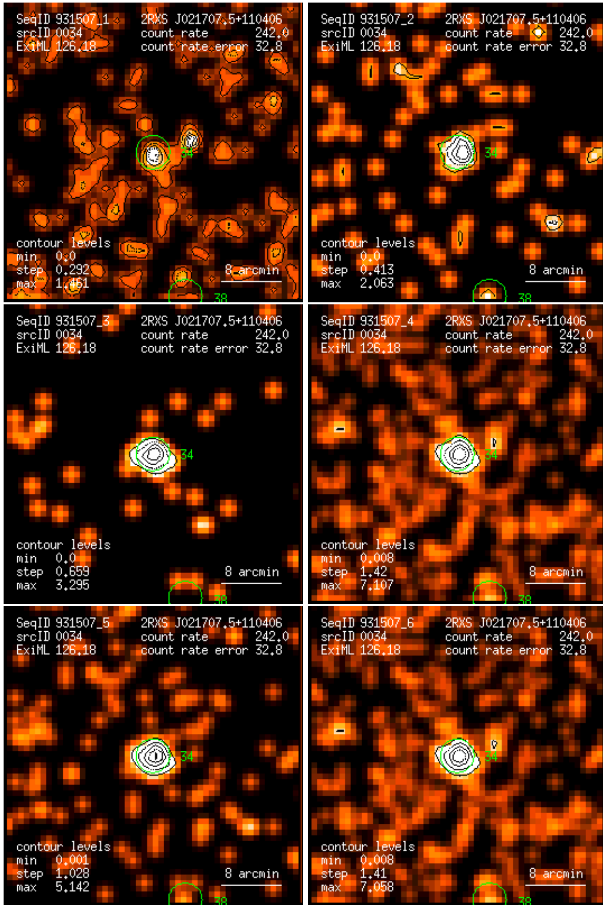
Figure 34: RASS 931507: detection 0034: band rate images, Gaussian filter: (1) PSPC channels 11 – 41, (2) 52 – 90, (3) 91 – 201, (4) 11 – 235, (5) 52 – 201, (6) 11 – 201. Broad band rates in counts/ks. Band rate contour levels in counts/ks/arcmin 2 .
