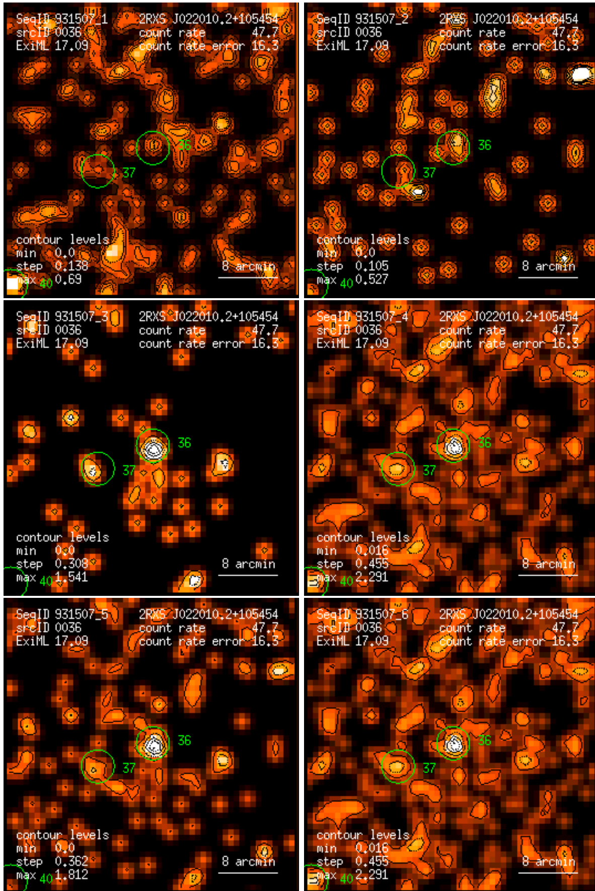
Figure 36: RASS 931507: detection 0036: band rate images, Gaussian filter: (1) PSPC channels 11 – 41, (2) 52 – 90, (3) 91 – 201, (4) 11 – 235, (5) 52 – 201, (6) 11 – 201. Broad band rates in counts/ks. Band rate contour levels in counts/ks/arcmin 2 .
