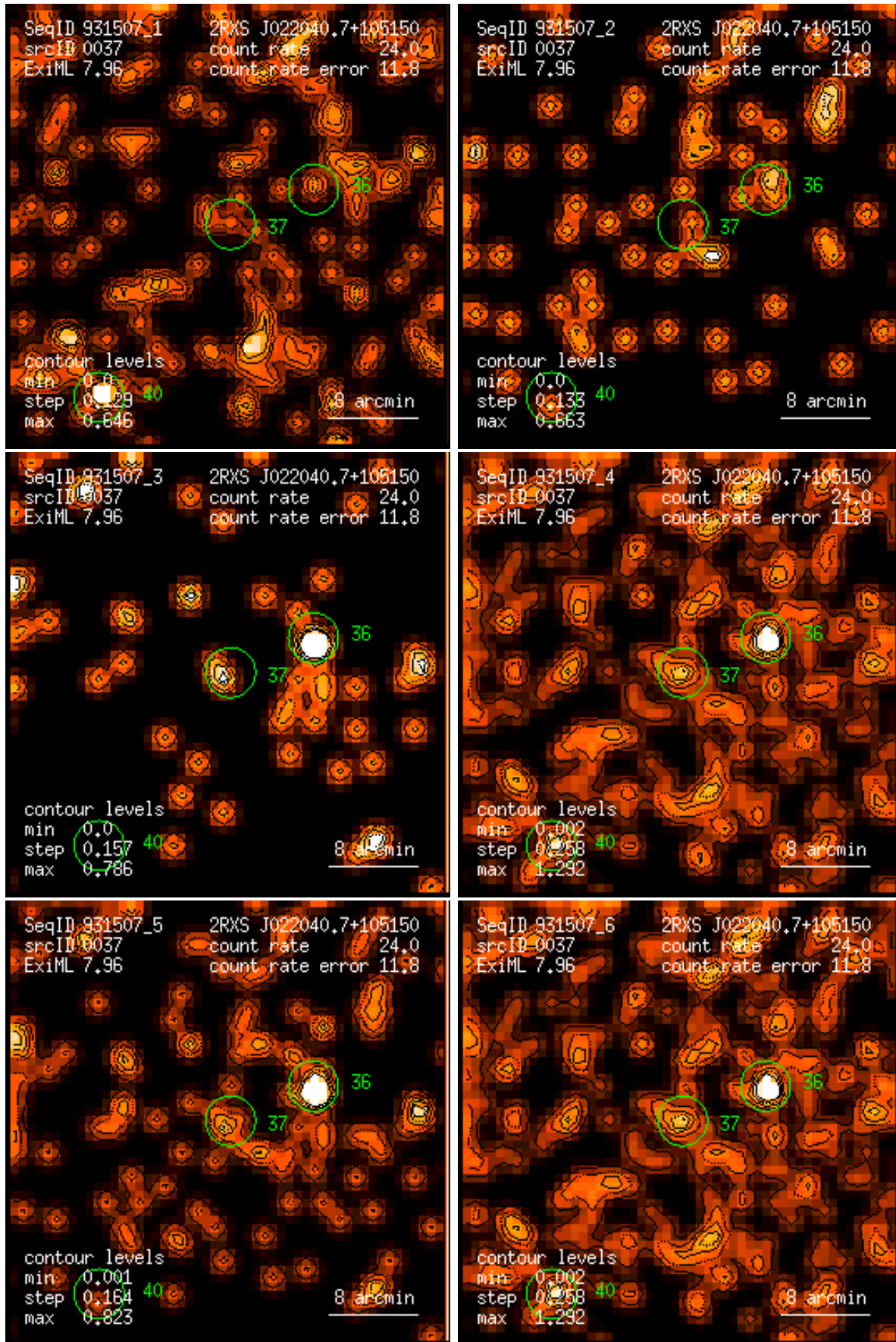
Figure 37: RASS 931507: detection 0037: band rate images, Gaussian filter: (1) PSPC channels 11 – 41, (2) 52 – 90, (3) 91 – 201, (4) 11 – 235, (5) 52 – 201, (6) 11 – 201. Broad band rates in counts/ks. Band rate contour levels in counts/ks/arcmin 2 .
