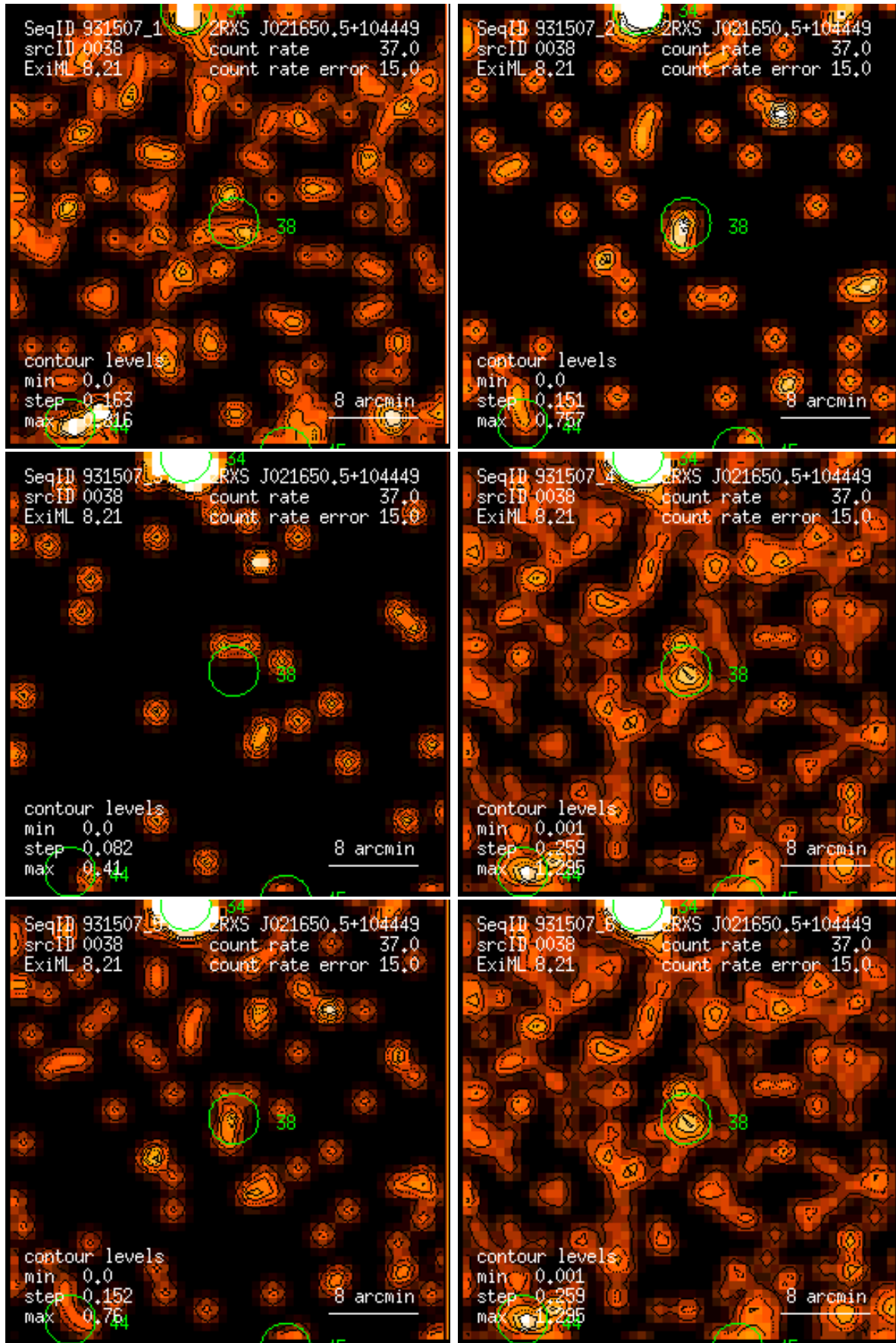
Figure 38: RASS 931507: detection 0038: band rate images, Gaussian filter: (1) PSPC channels 11 – 41, (2) 52 – 90, (3) 91 – 201, (4) 11 – 235, (5) 52 – 201, (6) 11 – 201. Broad band rates in counts/ks. Band rate contour levels in counts/ks/arcmin 2 .
