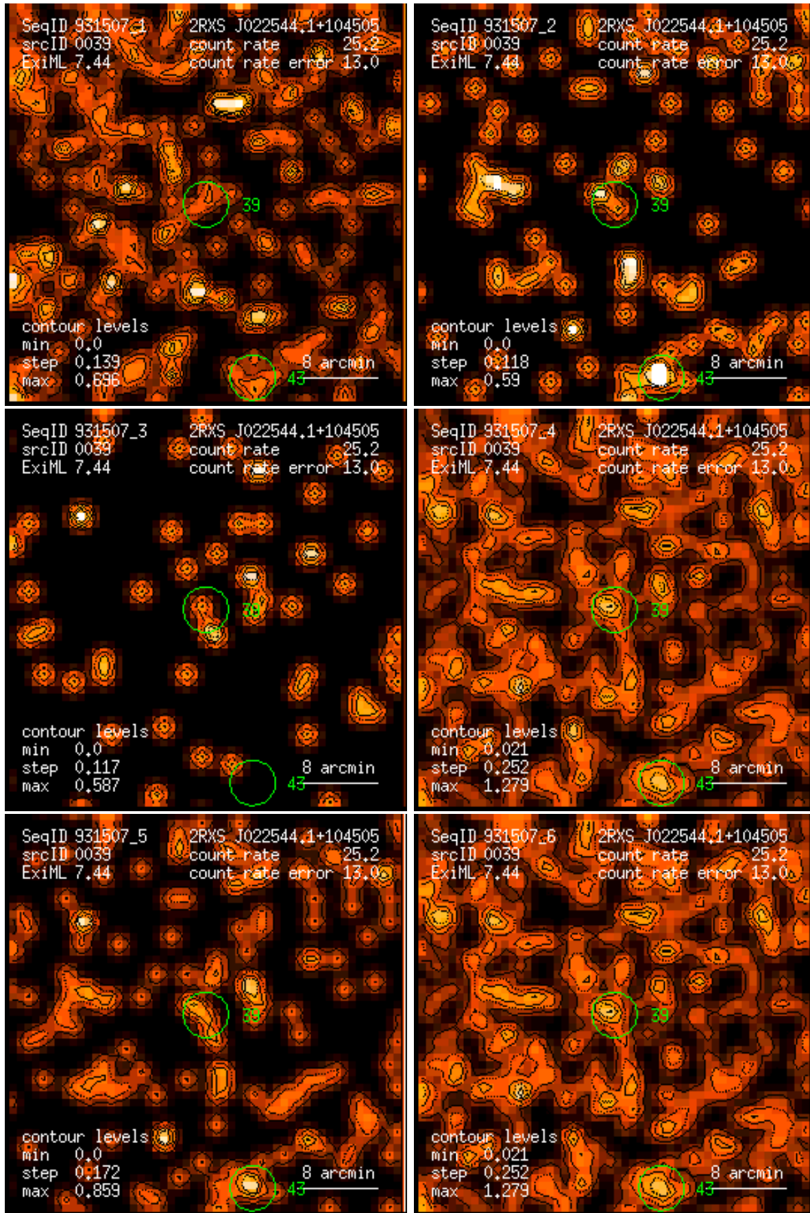
Figure 39: RASS 931507: detection 0039: band rate images, Gaussian filter: (1) PSPC channels 11 – 41, (2) 52 – 90, (3) 91 – 201, (4) 11 – 235, (5) 52 – 201, (6) 11 – 201. Broad band rates in counts/ks. Band rate contour levels in counts/ks/arcmin 2 .
