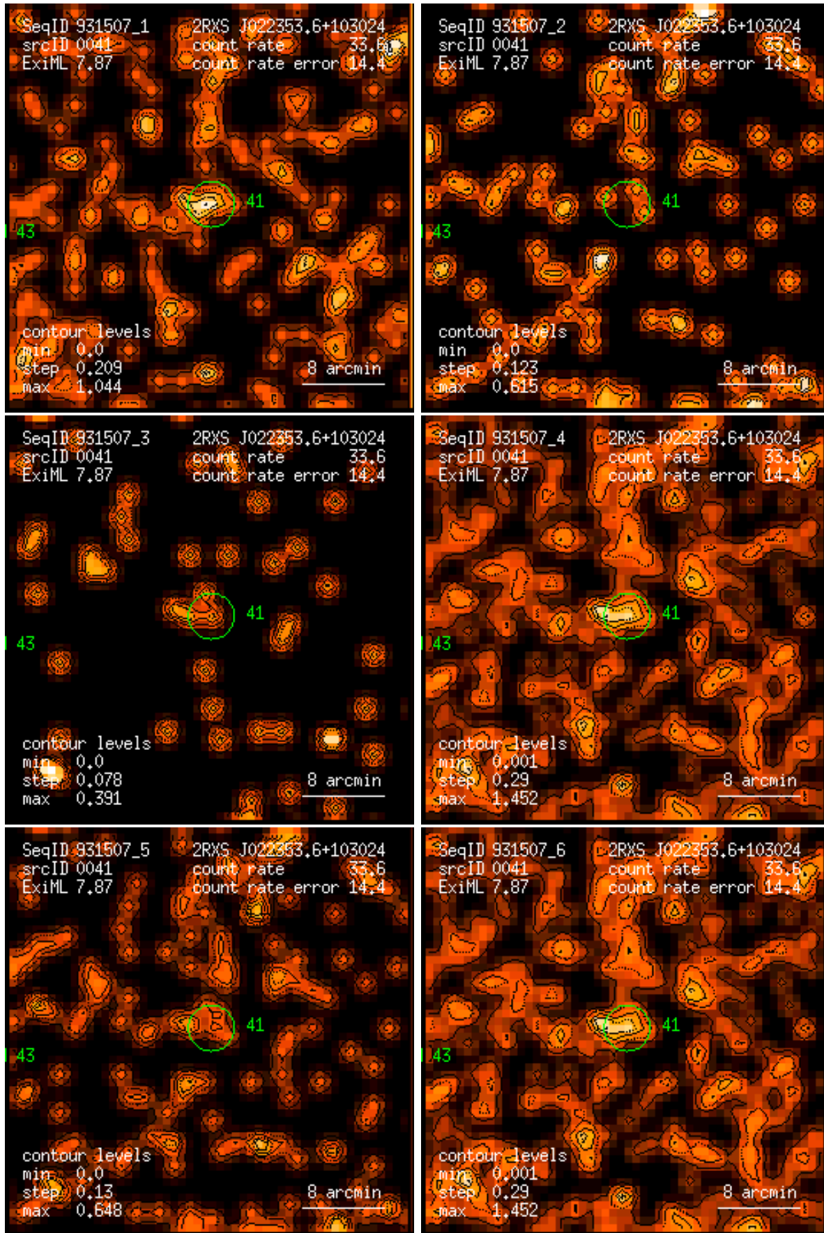
Figure 41: RASS 931507: detection 0041: band rate images, Gaussian filter: (1) PSPC channels 11 – 41, (2) 52 – 90, (3) 91 – 201, (4) 11 – 235, (5) 52 – 201, (6) 11 – 201. Broad band rates in counts/ks. Band rate contour levels in counts/ks/arcmin 2 .
