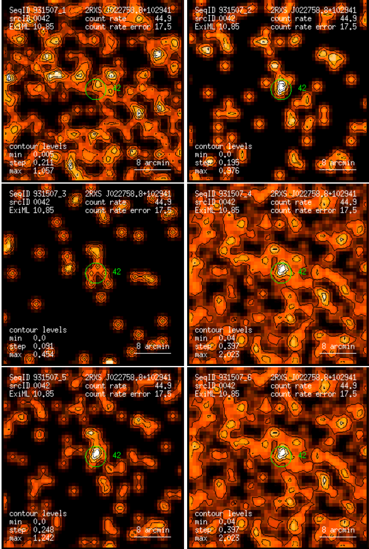
Figure 42: RASS 931507: detection 0042: band rate images, Gaussian filter: (1) PSPC channels 11 – 41, (2) 52 – 90, (3) 91 – 201, (4) 11 – 235, (5) 52 – 201, (6) 11 – 201. Broad band rates in counts/ks. Band rate contour levels in counts/ks/arcmin 2 .
