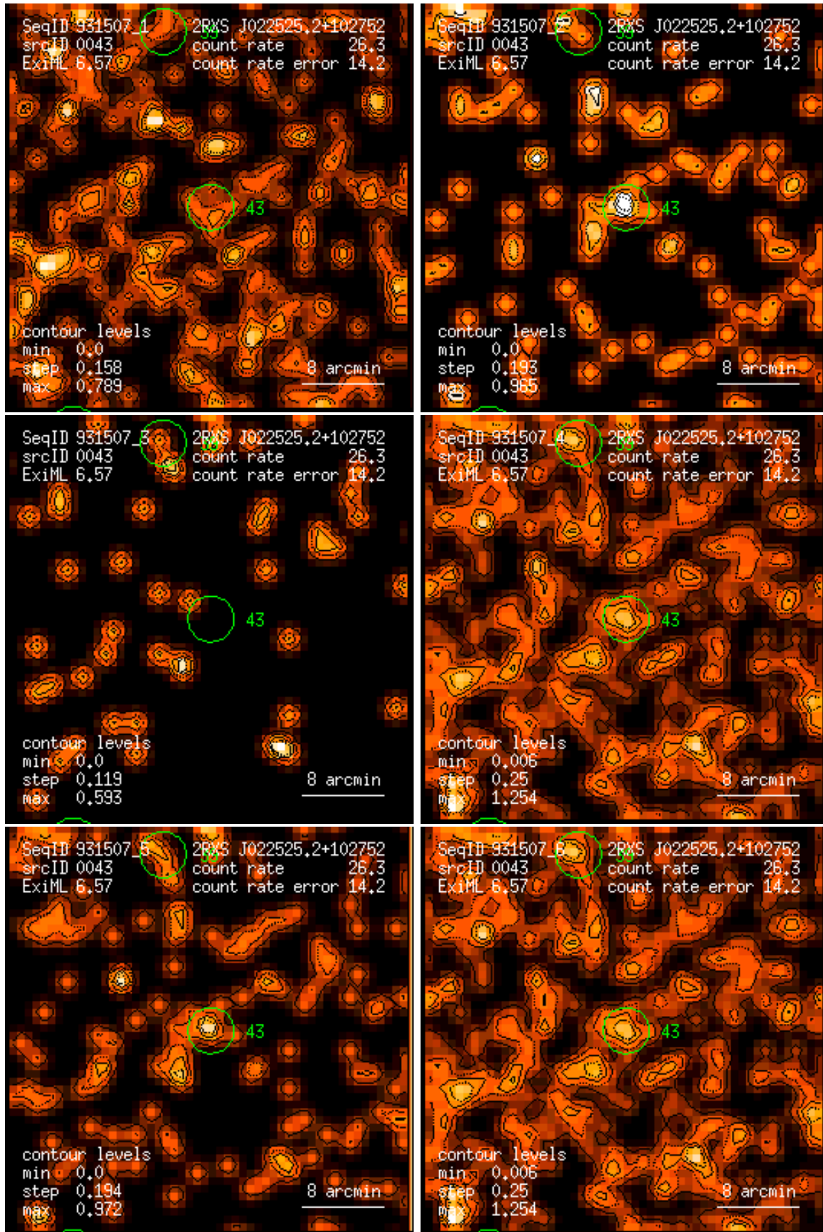
Figure 43: RASS 931507: detection 0043: band rate images, Gaussian filter: (1) PSPC channels 11 – 41, (2) 52 – 90, (3) 91 – 201, (4) 11 – 235, (5) 52 – 201, (6) 11 – 201. Broad band rates in counts/ks. Band rate contour levels in counts/ks/arcmin 2 .
