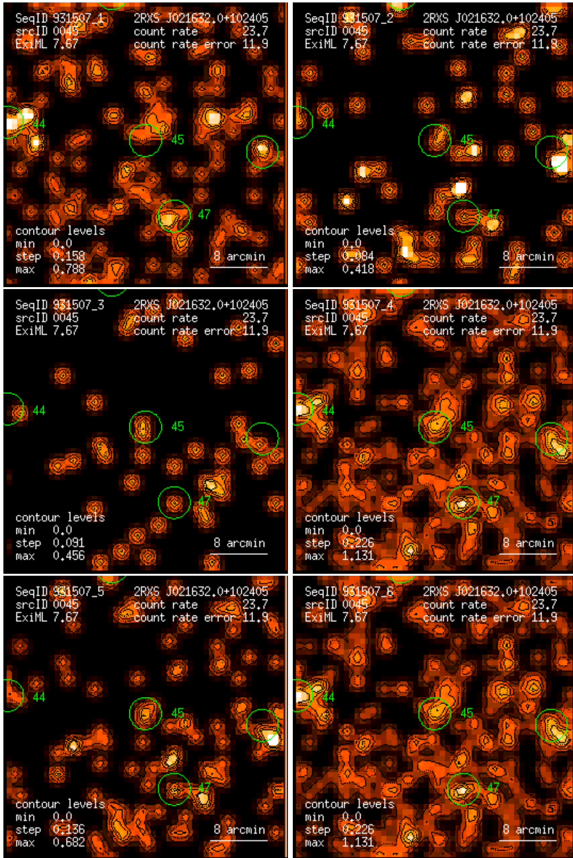
Figure 45: RASS 931507: detection 0045: band rate images, Gaussian filter: (1) PSPC channels 11 – 41, (2) 52 – 90, (3) 91 – 201, (4) 11 – 235, (5) 52 – 201, (6) 11 – 201. Broad band rates in counts/ks. Band rate contour levels in counts/ks/arcmin 2 .
