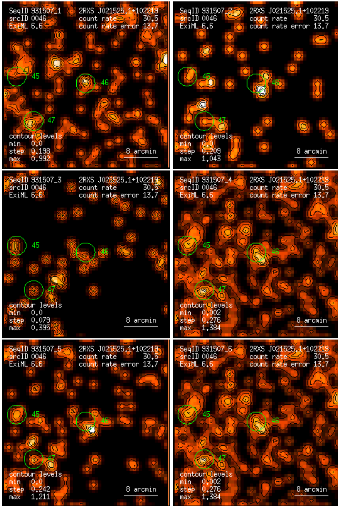
Figure 46: RASS 931507: detection 0046: band rate images, Gaussian filter: (1) PSPC channels 11 – 41, (2) 52 – 90, (3) 91 – 201, (4) 11 – 235, (5) 52 – 201, (6) 11 – 201. Broad band rates in counts/ks. Band rate contour levels in counts/ks/arcmin 2 .
