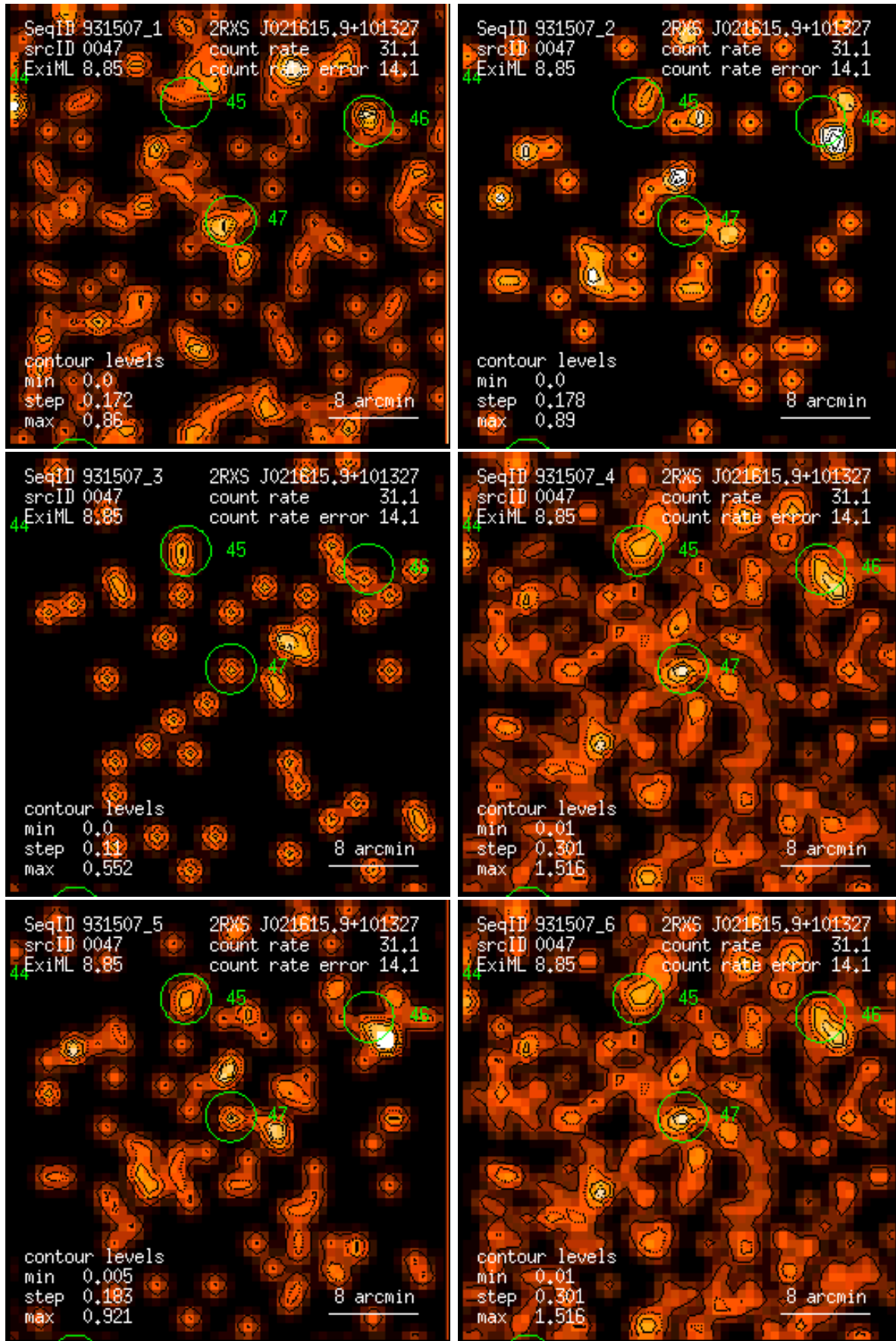
Figure 47: RASS 931507: detection 0047: band rate images, Gaussian filter: (1) PSPC channels 11 – 41, (2) 52 – 90, (3) 91 – 201, (4) 11 – 235, (5) 52 – 201, (6) 11 – 201. Broad band rates in counts/ks. Band rate contour levels in counts/ks/arcmin 2 .
