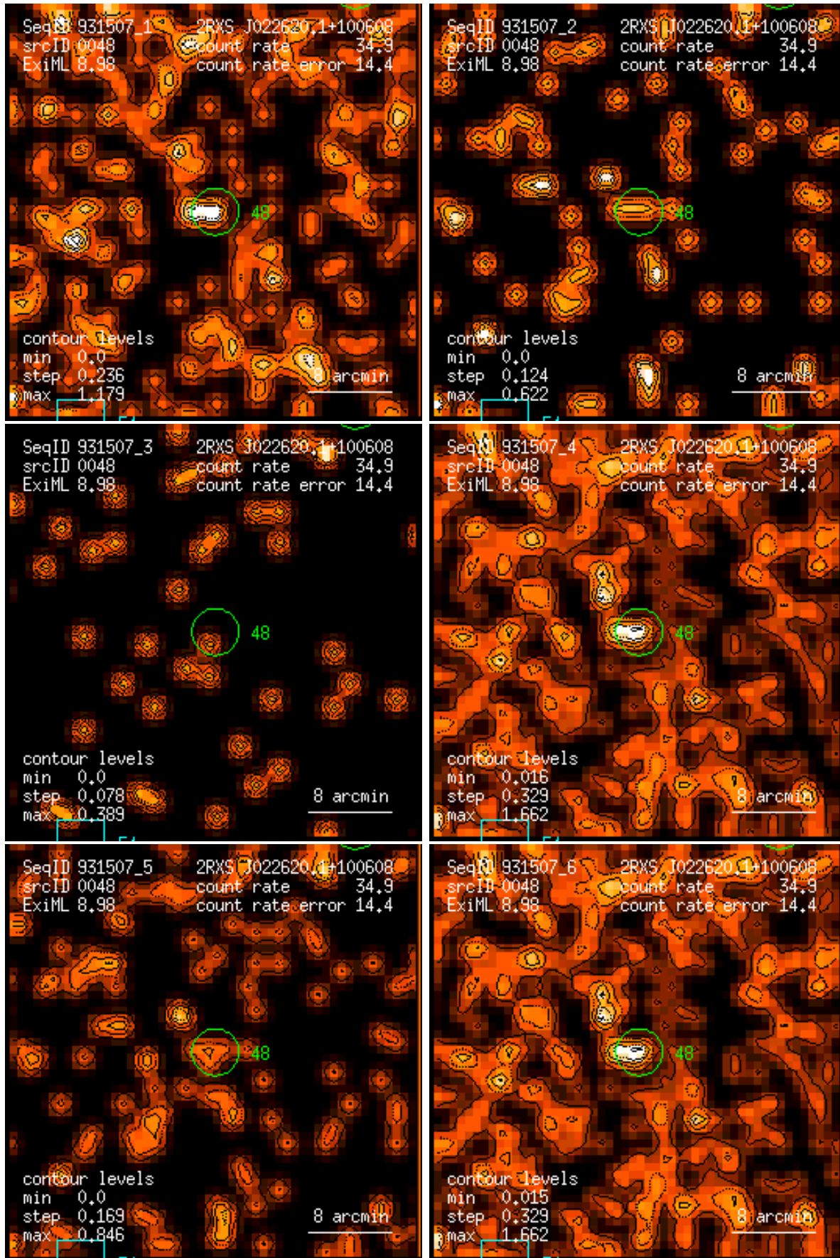
Figure 48: RASS 931507: detection 0048: band rate images, Gaussian filter: (1) PSPC channels 11 – 41, (2) 52 – 90, (3) 91 – 201, (4) 11 – 235, (5) 52 – 201, (6) 11 – 201. Broad band rates in counts/ks. Band rate contour levels in counts/ks/arcmin 2 .
