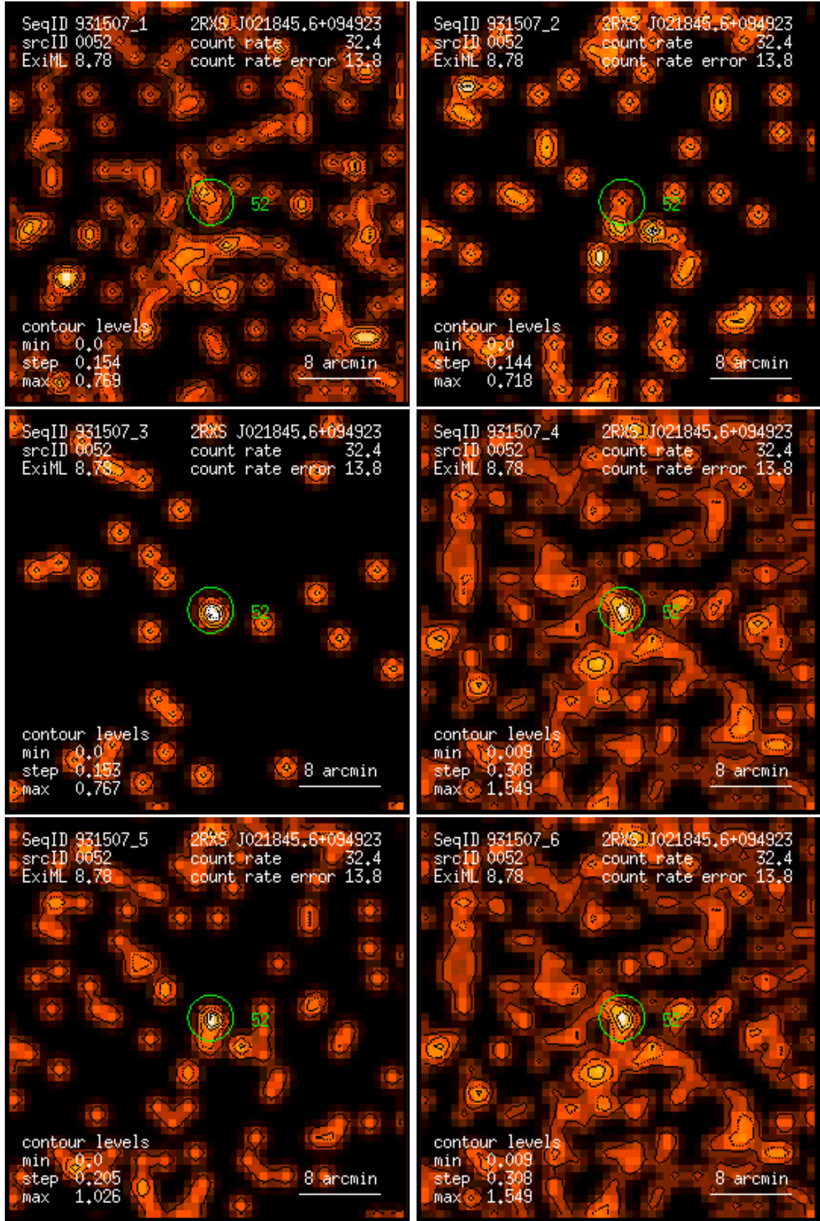
Figure 52: RASS 931507: detection 0052: band rate images, Gaussian filter: (1) PSPC channels 11 – 41, (2) 52 – 90, (3) 91 – 201, (4) 11 – 235, (5) 52 – 201, (6) 11 – 201. Broad band rates in counts/ks. Band rate contour levels in counts/ks/arcmin 2 .
