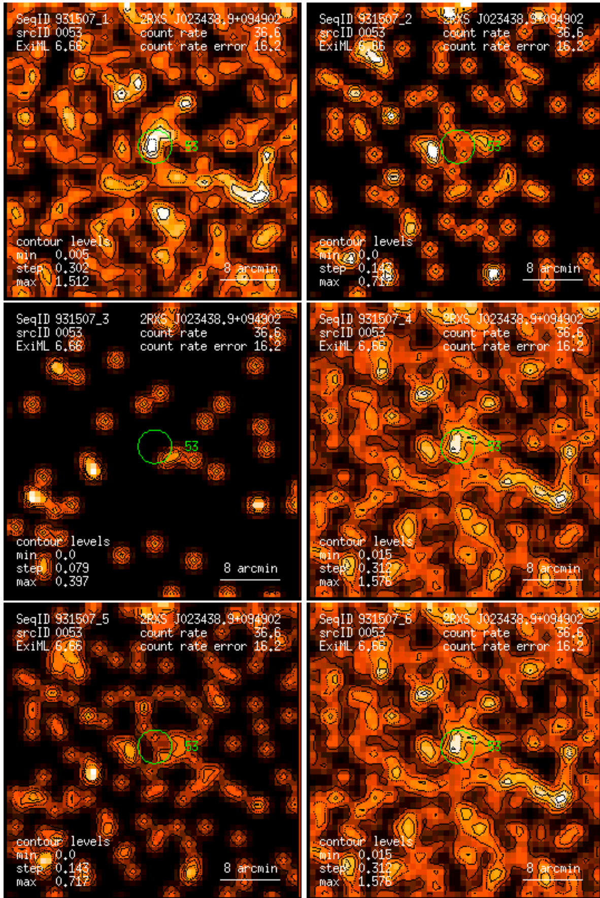
Figure 53: RASS 931507: detection 0053: band rate images, Gaussian filter: (1) PSPC channels 11 – 41, (2) 52 – 90, (3) 91 – 201, (4) 11 – 235, (5) 52 – 201, (6) 11 – 201. Broad band rates in counts/ks. Band rate contour levels in counts/ks/arcmin 2 .
