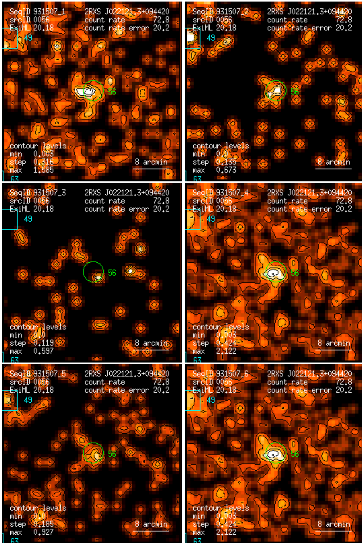
Figure 56: RASS 931507: detection 0056: band rate images, Gaussian filter: (1) PSPC channels 11 – 41, (2) 52 – 90, (3) 91 – 201, (4) 11 – 235, (5) 52 – 201, (6) 11 – 201. Broad band rates in counts/ks. Band rate contour levels in counts/ks/arcmin 2 .
