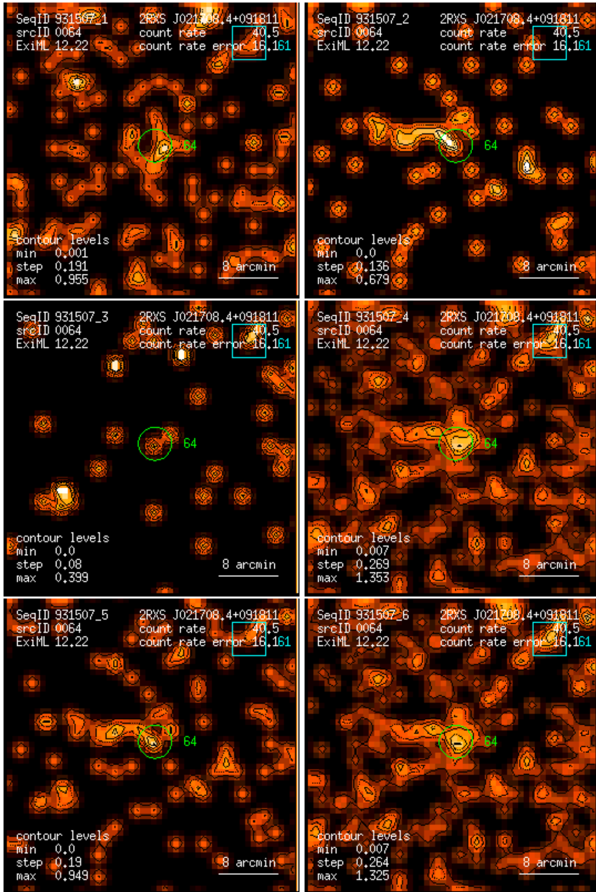
Figure 64: RASS 931507: detection 0064: band rate images, Gaussian filter: (1) PSPC channels 11 – 41, (2) 52 – 90, (3) 91 – 201, (4) 11 – 235, (5) 52 – 201, (6) 11 – 201. Broad band rates in counts/ks. Band rate contour levels in counts/ks/arcmin 2 .
