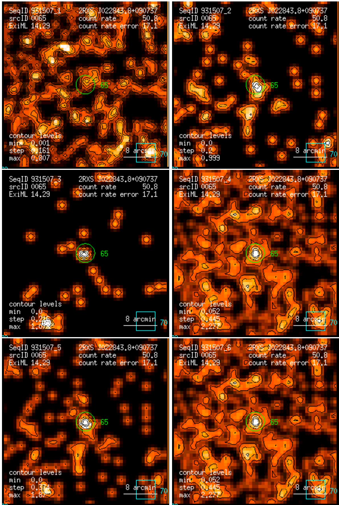
Figure 65: RASS 931507: detection 0065: band rate images, Gaussian filter: (1) PSPC channels 11 – 41, (2) 52 – 90, (3) 91 – 201, (4) 11 – 235, (5) 52 – 201, (6) 11 – 201. Broad band rates in counts/ks. Band rate contour levels in counts/ks/arcmin 2 .
