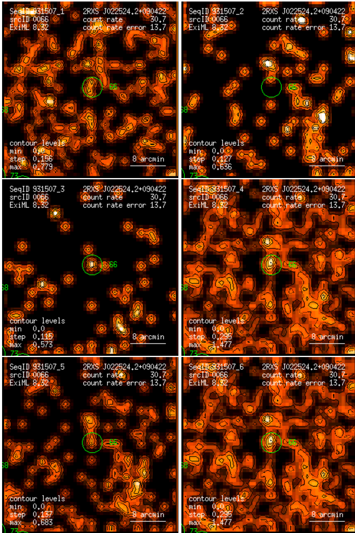
Figure 66: RASS 931507: detection 0066: band rate images, Gaussian filter: (1) PSPC channels 11 – 41, (2) 52 – 90, (3) 91 – 201, (4) 11 – 235, (5) 52 – 201, (6) 11 – 201. Broad band rates in counts/ks. Band rate contour levels in counts/ks/arcmin 2 .
