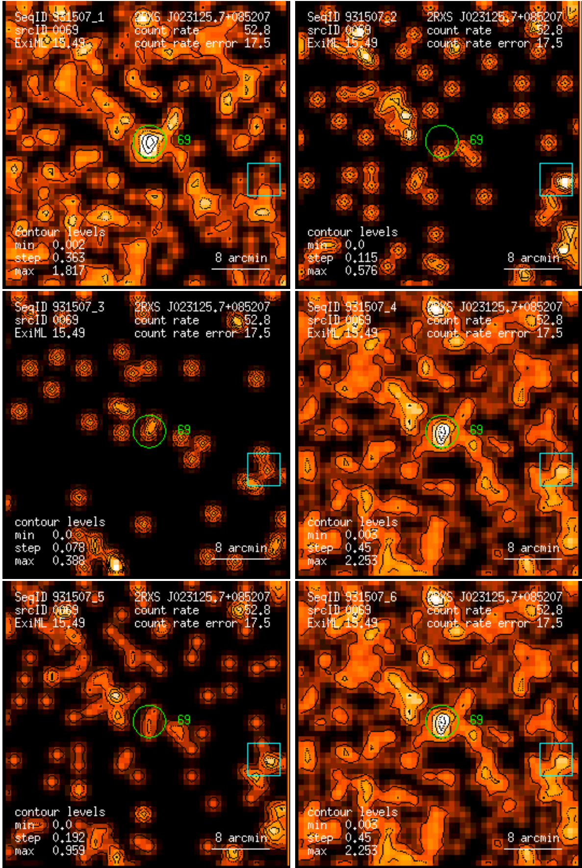
Figure 69: RASS 931507: detection 0069: band rate images, Gaussian filter: (1) PSPC channels 11 – 41, (2) 52 – 90, (3) 91 – 201, (4) 11 – 235, (5) 52 – 201, (6) 11 – 201. Broad band rates in counts/ks. Band rate contour levels in counts/ks/arcmin 2 .
