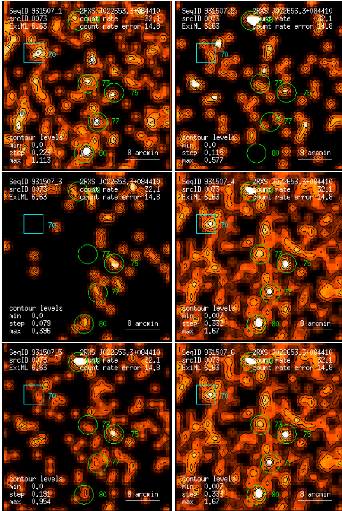
Figure 73: RASS 931507: detection 0073: band rate images, Gaussian filter: (1) PSPC channels 11 – 41, (2) 52 – 90, (3) 91 – 201, (4) 11 – 235, (5) 52 – 201, (6) 11 – 201. Broad band rates in counts/ks. Band rate contour levels in counts/ks/arcmin 2 .
