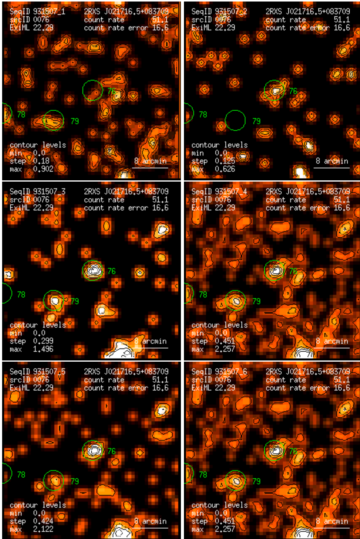
Figure 76: RASS 931507: detection 0076: band rate images, Gaussian filter: (1) PSPC channels 11 – 41, (2) 52 – 90, (3) 91 – 201, (4) 11 – 235, (5) 52 – 201, (6) 11 – 201. Broad band rates in counts/ks. Band rate contour levels in counts/ks/arcmin 2 .
