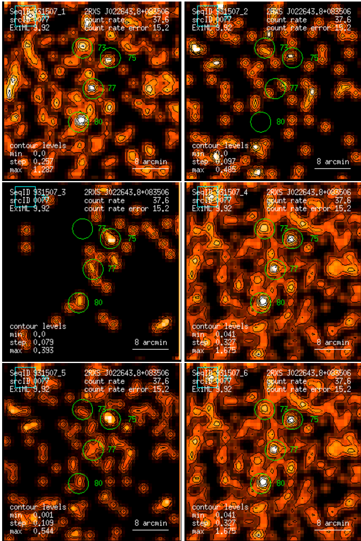
Figure 77: RASS 931507: detection 0077: band rate images, Gaussian filter: (1) PSPC channels 11 – 41, (2) 52 – 90, (3) 91 – 201, (4) 11 – 235, (5) 52 – 201, (6) 11 – 201. Broad band rates in counts/ks. Band rate contour levels in counts/ks/arcmin 2 .
