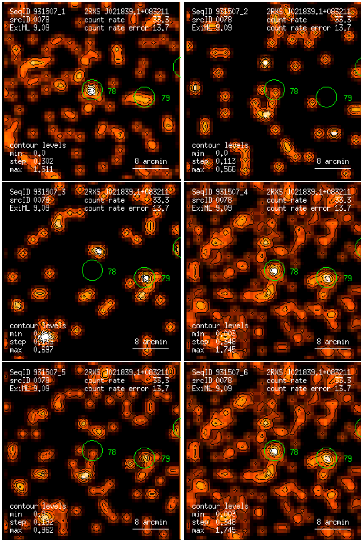
Figure 78: RASS 931507: detection 0078: band rate images, Gaussian filter: (1) PSPC channels 11 – 41, (2) 52 – 90, (3) 91 – 201, (4) 11 – 235, (5) 52 – 201, (6) 11 – 201. Broad band rates in counts/ks. Band rate contour levels in counts/ks/arcmin 2 .
