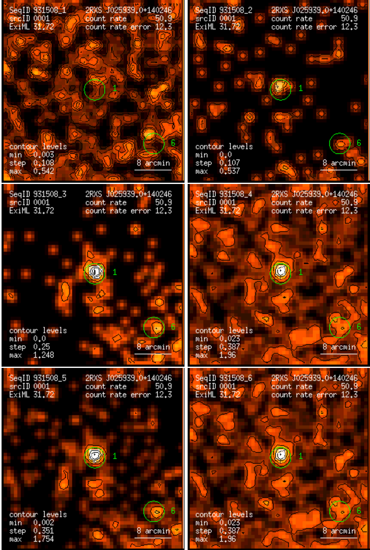
Figure 1: RASS 931508: detection 0001: band rate images, Gaussian filter: (1) PSPC channels 11 – 41, (2) 52 – 90, (3) 91 – 201, (4) 11 – 235, (5) 52 – 201, (6) 11 – 201. Broad band rates in counts/ks. Band rate contour levels in counts/ks/arcmin 2 .
