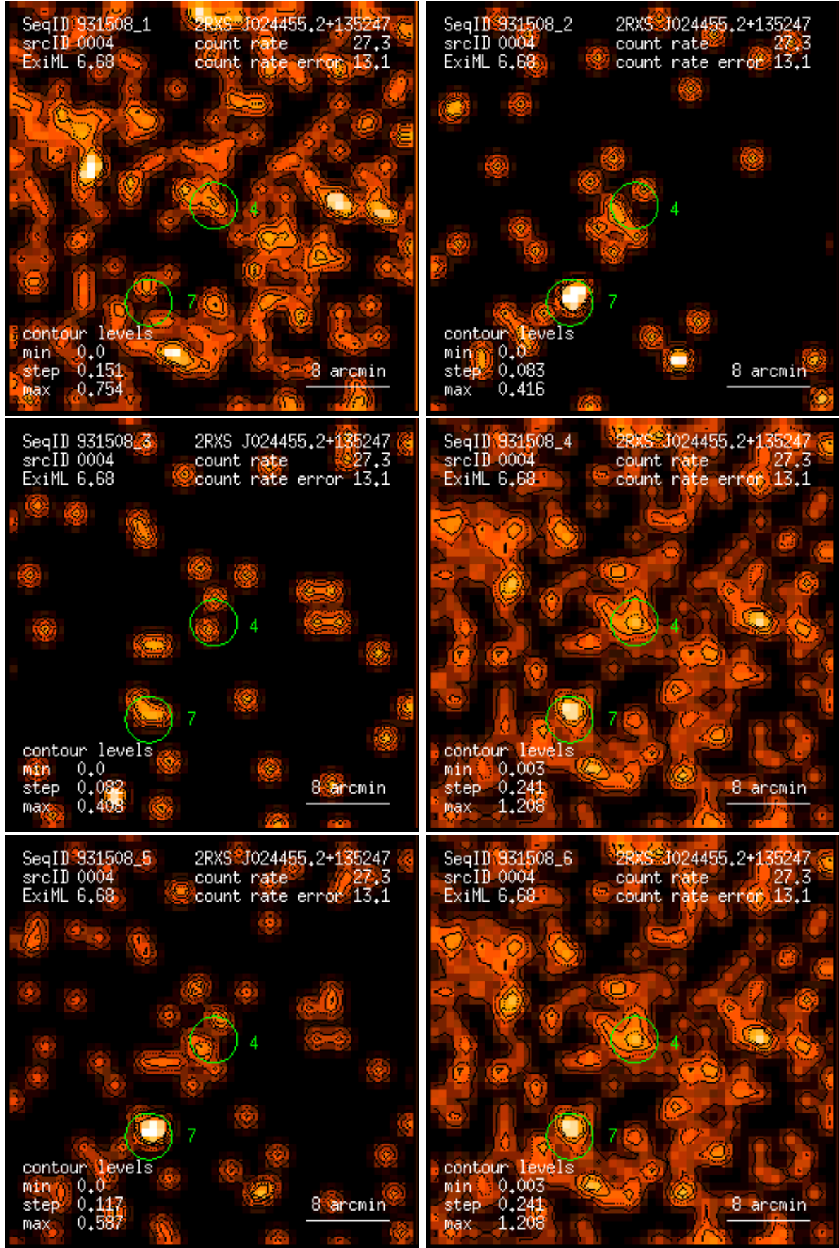
Figure 4: RASS 931508: detection 0004: band rate images, Gaussian filter: (1) PSPC channels 11 – 41, (2) 52 – 90, (3) 91 – 201, (4) 11 – 235, (5) 52 – 201, (6) 11 – 201. Broad band rates in counts/ks. Band rate contour levels in counts/ks/arcmin 2 .
